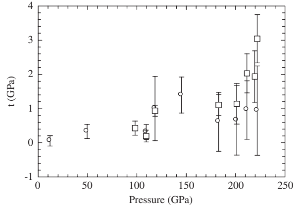
Fig. 8. The pressure dependence of t obtained using line-shift data (unfilled squares) and line-width data (unfilled circles).
