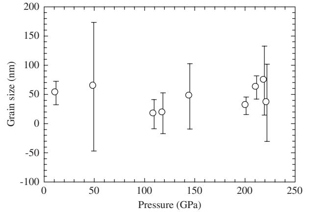
Fig. 4. The grain sizes at different pressures.
