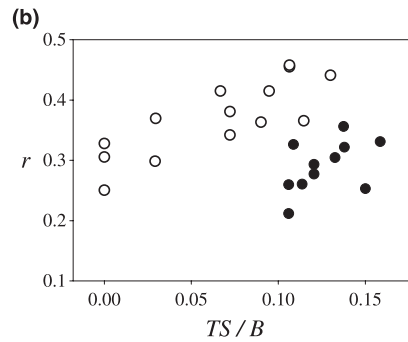
Fig. 2 Main morphological responses of Daphnia at their age of first reproduction, in relation with their calculated population growth rate ( r ). Empty and filled circles show control and kairomone treatments respectively: (a) body length and tail spine length versus r , (b) ratio of tail spine length to body length versus r . Correlation is significant (Spearman's rank test, P < 0.05 ) only for controls.
