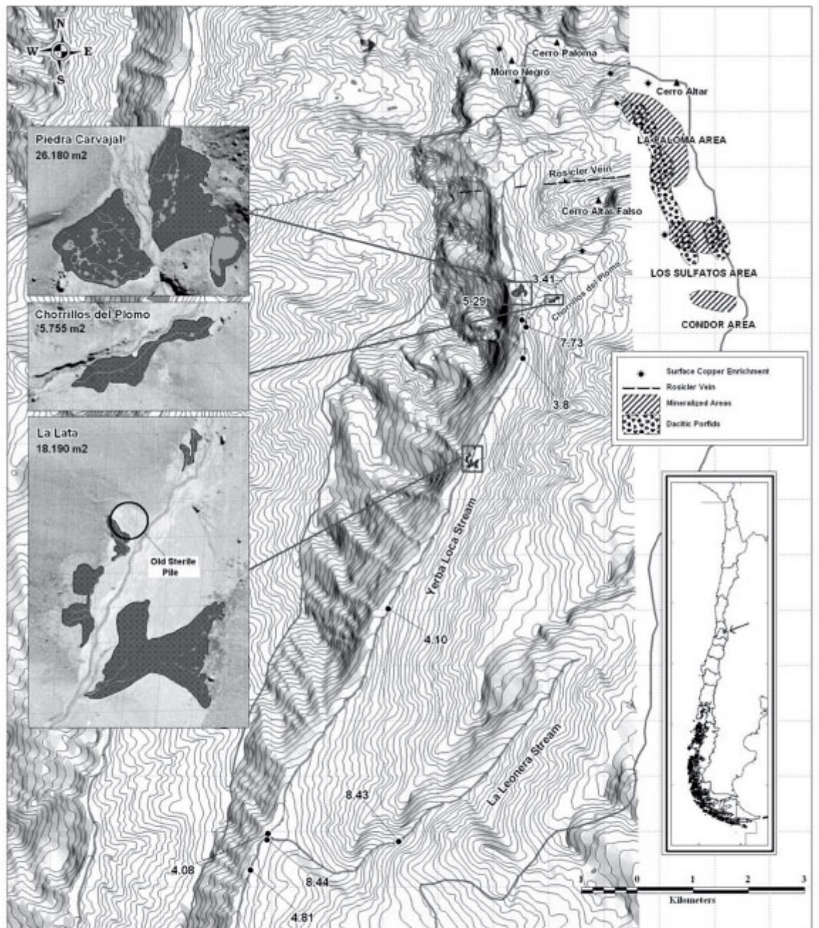
Fig. 1: Location of Yerba Loca Natural Sanctuary (YLNS) in central Chile. Relative distribution of study high-alpine meadows, high-altitude mineral deposits and abandoned sterile pile from historic small-scale silver exploitation is indicated. Numbers in the map indicate pH values of surface water.
