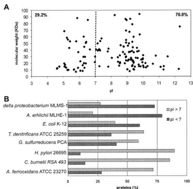
FIG. 3. pI distribution among periplasmic proteins found in A. ferrooxidans compared with some other Gram-negative microorganisms. A, distribution of all proteins found in the periplasmic fraction from A. ferrooxidans ATCC 23270 grown in thiosulfate according to their theoretical molecular masses and isoelectric points. B, percentage of SignalP or TatP proteins with pI values above and below 7.0 predicted in complete genomes of Gram-negative bacteria. Alkalophiles, delta -proteobacterium MLMS-1 and A. ehrlichii MLHE-1; neutrophiles, E. coli K-12, T. denitrificans ATCC 25259, and G. sulfurreducens PCA; acidophiles, C. burnetii RSA 493 and A. ferrooxidans ATCC 23270. Also included in this group for comparison is the acid-tolerant H. pylori 26695.
