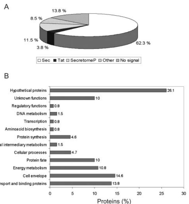
FIG. 2. Global analysis of periplasmic proteins from A. ferrooxidans . A, percent distribution of proteins according to their export signals. B, distribution of periplasmic proteins in functional categories according to TIGR annotation.
