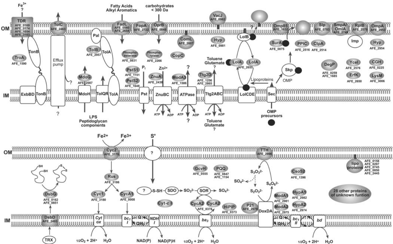
FIG. 4. Schematic location and suggested putative functions of the majority of the proteins identified in the periplasmic fraction from A. ferrooxidans . Most of the proposed localizations and possible roles of the indicated proteins are based on previously reported studies in E. coli and other microorganisms (1, 33, 40, 43, 73). The proteins shaded in gray were identified experimentally by proteomics analysis of the periplasmic fraction. Transport functions are highlighted in the upper part, and energy metabolism is in the lower portion of the figure. The OMPs are shown in their final destination into the outer membrane. Black circles represent OMP precursors in transit to the outer membrane. The order in which the different proteins are included in this schematic is arbitrary.
