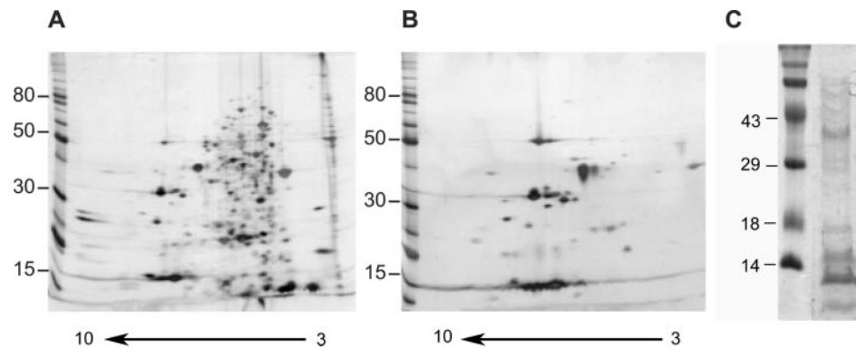
FIG. 1. 2-D PAGE of the periplasmic fraction of A. ferrooxidans grown on thiosulfate. Total proteins (A) or periplasmic fraction (B and C) were separated by 2-D NEPHGE (A and B) with a pH gradient between 3.0 (right side of the gel) and 10.0 (left side of the gel) or by monodimensional SDS-PAGE (C). Spots were detected by silver stain (A and B) or by colloidal Coomassie Blue (C). Molecular mass standards (in kilodaltons) are given on the left of the gels.
