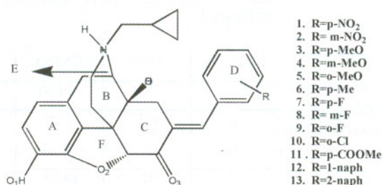
Figure 1. 7-Arylidenenaltrexones.
