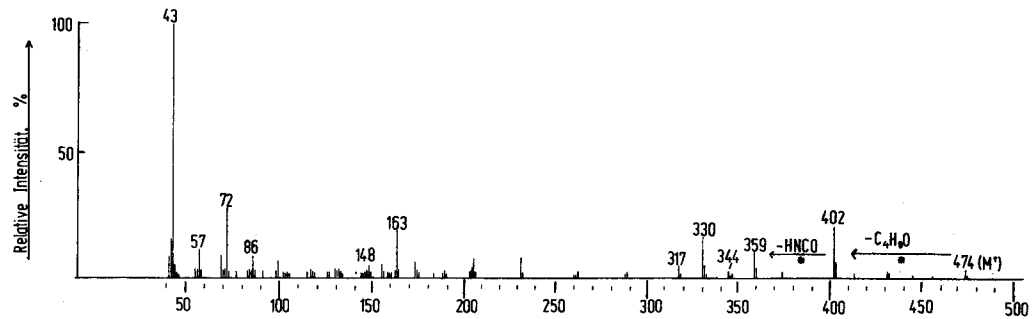
Fig 1. Mass spectrum of zizyphine-D (6).
