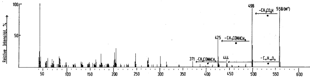
Fig 2. Mass spectrum of N,O-diacetyl-zizyphine-D.
