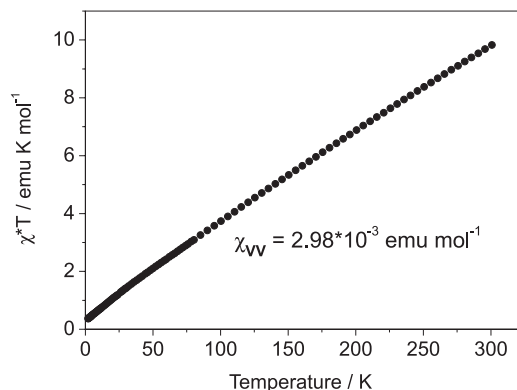
Figure 5. \chi^*T versus T diagram: Van Vleck term ( \chi_{VV} ) was estimated in the high temperature range ( 150 \leq T \leq 300 K).
