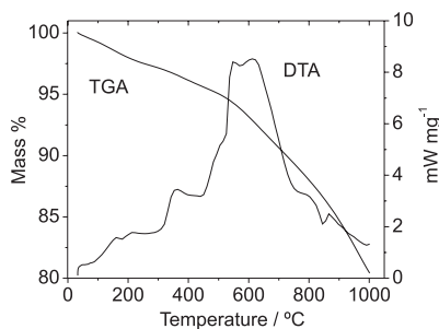
Figure 3. DTA/TGA profiles of K_2SmP_2S_7 .
