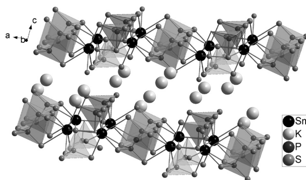
Figure 1. Crystal structure of K_2SmP_2S_7 down the b -axis.
