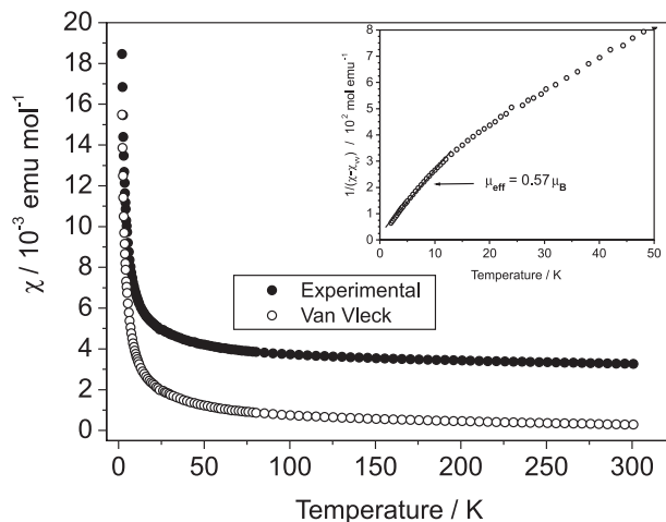
Figure 6. Magnetic susceptibility measured under 2.5 kOe: filled symbols represent the experimental data; empty symbols show data after correction of a Van Vleck term ( \chi_{VV} ). The insert shows the corrected inverse susceptibility and an estimation of the effective magnetic moment on the low temperature range.
