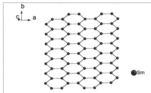
Figure 2. Arrangement of Sm^{3+} cations in one layer.
