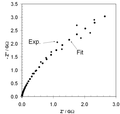
Figure 4. Impedance-frequency measurement. Average of 5 measurements, taken at 313.3 K.
