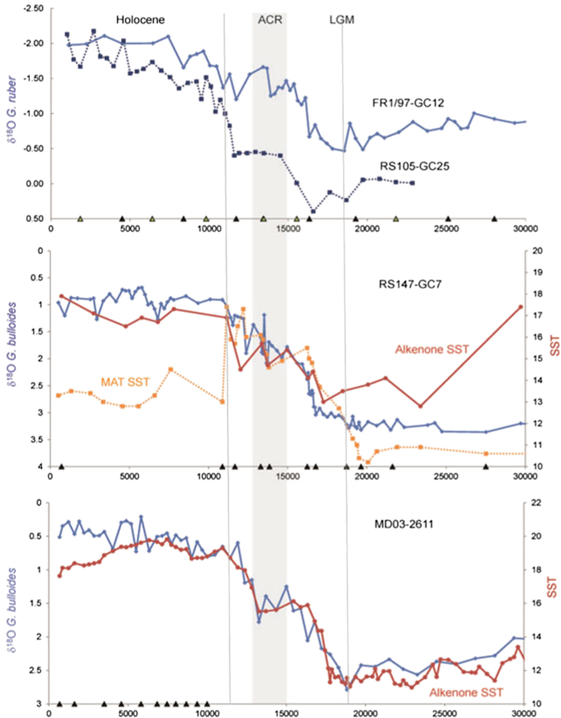
Fig. 4. Top graph shows the \delta^{18}\text{O} G. ruber records of FR1/97-GC12 (Bostock et al., 2006) and RS105-GC25 (Troedson and Davies, 2001). The middle graph shows the \delta^{18}\text{O} G. bulloides (blue) and foraminiferal assemblage MAT SST (orange) and alkenone SST (red) from core RS147-GC7 (Sikes et al., 2009). The bottom graph shows the \delta^{18}\text{O} G. bulloides (blue) and alkenone SST (red) from MD03-2611 (Calvo et al., 2007; Gingele et al., 2007). The black triangles highlight the radiocarbon samples (green triangles for RS105-GC7). The LGM determined by maximum in \delta^{18}\text{O} in most of the cores at ~19 ka is highlighted by a dashed grey line. The ACR is highlighted by a grey box from 12.5 to 15 ka, the start of the Holocene is shown by a grey dashed line at ~11.5 ka.
