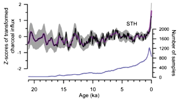
Fig. 6. Macrocharcoal composite from the modern subtropical high pressure belt (STH: 25°S–45°S, 100°E–177°W, broadly temperate Australasia). The data have been smoothed using a window of 400 years (purple line) and a window of 100 years (bold black line) to emphasize the centennial-scale variability. The bootstrapped confidence intervals are based on a 400-year smoothing of the curves. The number of observations contributing to the record within each 400-year window is also shown (blue line) (Mooney et al., 2011).
