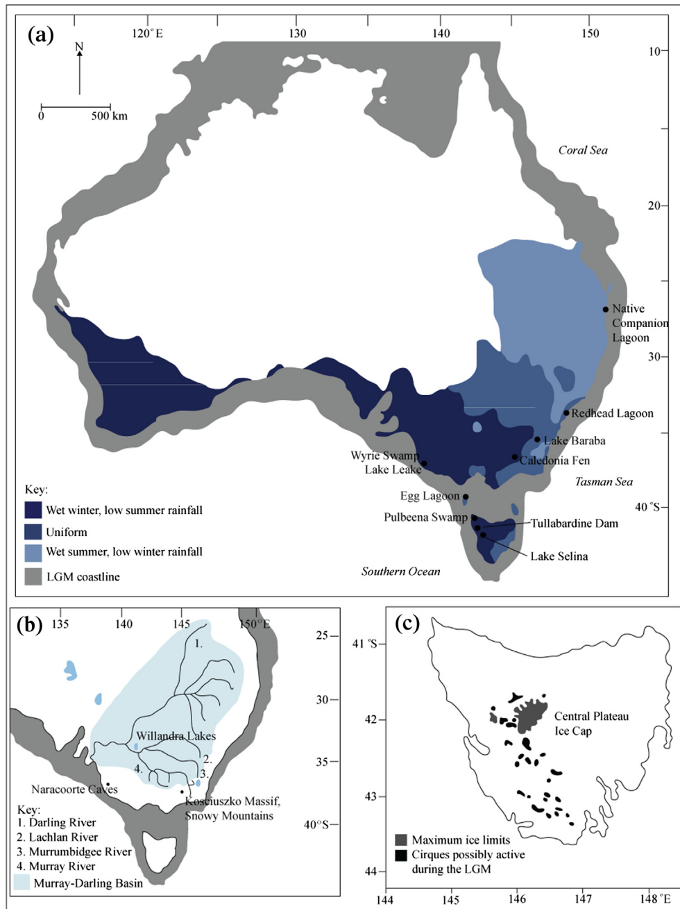
Fig. 1. Location of continuous records of climatic and environmental variability encompassing the period 30–0 ka in eastern Australia, (a) overlain on rainfall seasonality in the temperate zone (adapted from BOM, 2005) with the estimated LGM coastline (adapted from Gillespie, 2002), (b) the hydrologic and fluvial record sites in the Murray–Darling Basin along with the location of the Naracoorte Caves and the Kosciuszko Massif, and (c) close-up of Tasmania showing the extent of glacialiation during the late Pleistocene (adapted from Barrows et al., 2002).
