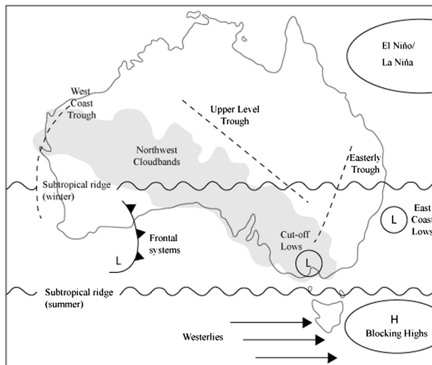
Fig. 3. Modern drivers of climate variability in temperate Australia (adapted from BOM, 2005; Risbey et al., 2009).
