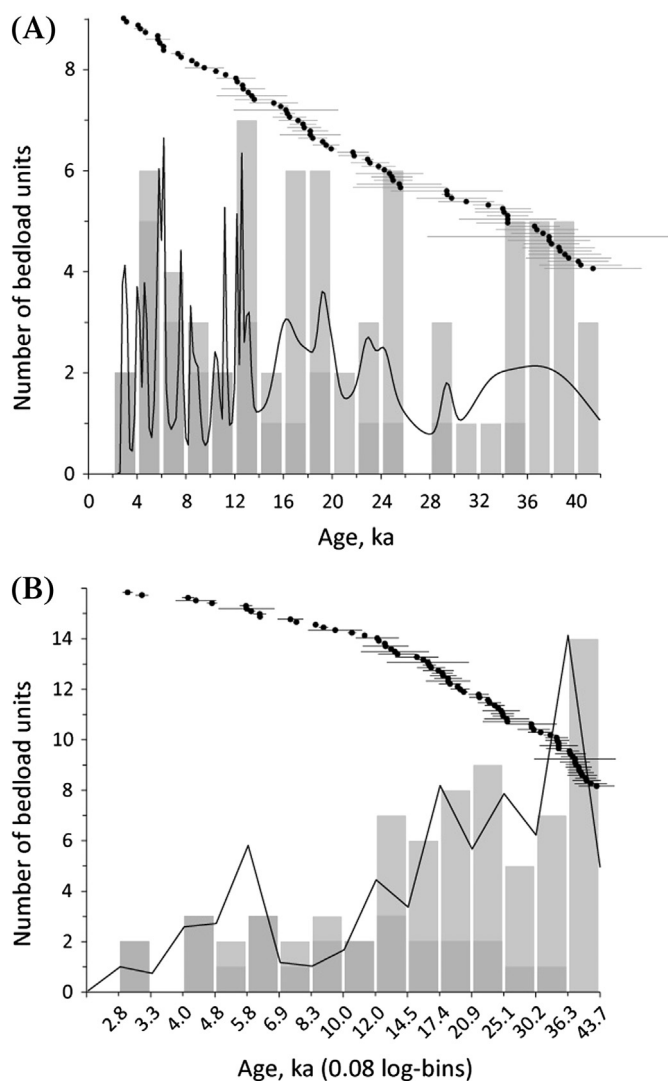
Fig. 5. Compilation of OSL, TL and ^{14}\text{C} -dated bedload units from rivers in the Murray–Darling Basin plotted as frequency distributions of depositional ages ( n = 73 ); (A) Ranked age plot with 1\sigma errors, histogram (linear 2 ka bins) and kernel density estimate (0.2 ka bandwidth) plotted as non-dimensional probability, and (B) The same data separated into 0.08 logarithmic bins, which expand with age as indicated, and kernel density estimate (0.08 log ka bandwidth) plotted as non-dimensional probability. ^{14}\text{C} dates are denoted by dark-grey shading in the histograms (Bowler, 1978; Bowler et al., 1978; Page et al., 1991; Page and Nanson, 1996; Ogden et al., 2001; Kemp and Spooner, 2007; dated units derived from; Power et al., 2008; Kemp and Rhodes, 2010). Ages <2 ka are excluded and the weighted mean age is plotted for bedload units with multiple dates.
