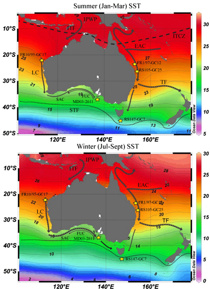
Fig. 2. Map of the modern SST for Austral summer (Jan–Mar) and Austral winter (Jul–Sept) with the position of the main surface currents and subtropical front. The location of the main cores described in the text and in this figure is shown by a yellow star. EAC – East Australian Current, LC – Leeuwin Current, FUC – Flinders Undercurrent, TF – Tasman Front, STF – Subtropical Front, ITCZ – Inter-tropical Convergence Zone.
