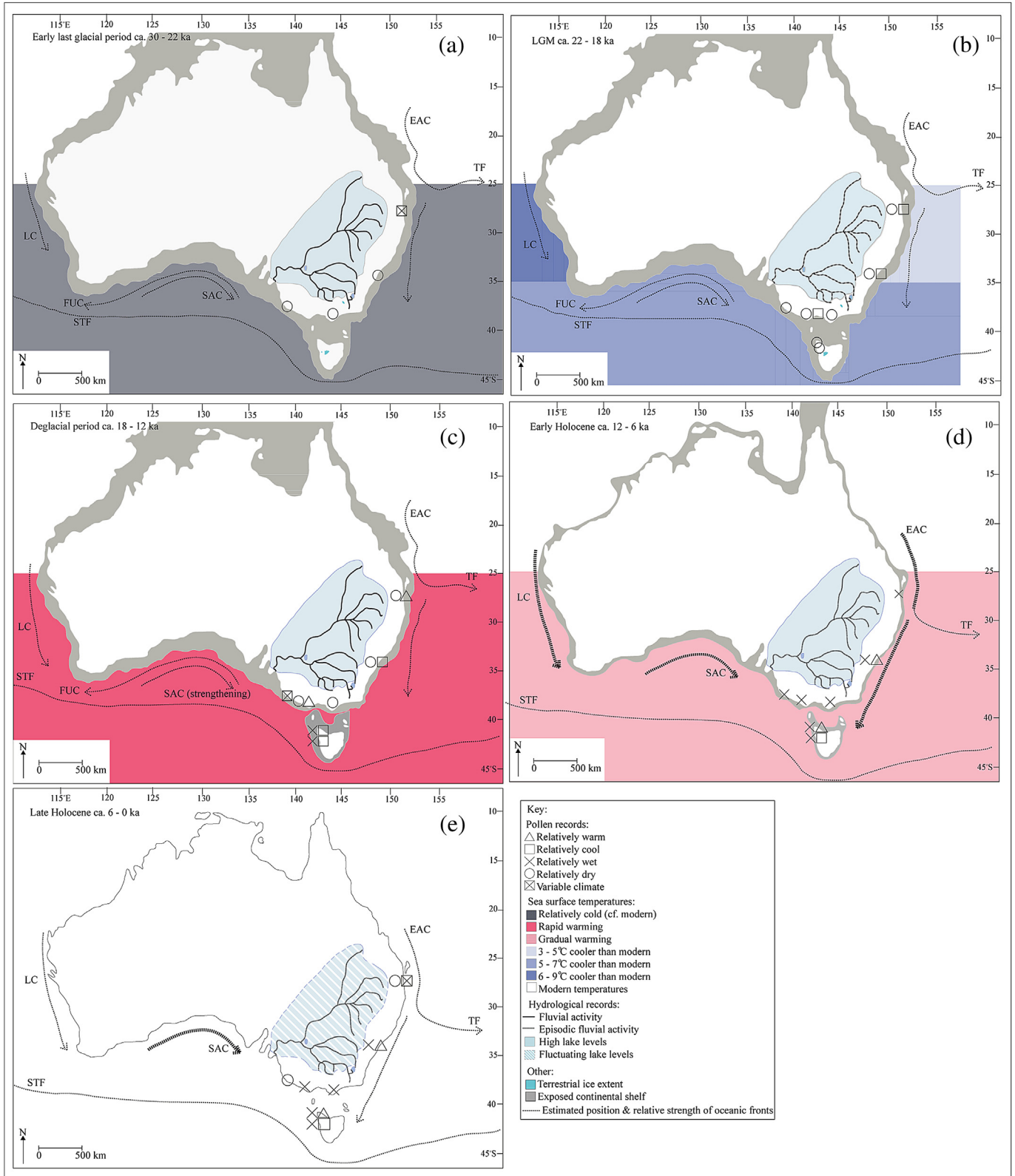
Fig. 7. Comparison of climatic conditions indicated by proxy records from temperate Australia for the periods (a) early Last Glacial period, (b) LGM, (c) the deglacial period, (d) early to mid-Holocene and (e) mid to late Holocene, indicating the position of oceanic fronts and currents (Martinez, 1994; Passlow et al., 1997; Martinez et al., 1999; Troedson and Davies, 2001; Barrows and Juggins, 2005; Bostock et al., 2006; Pelejero et al., 2006; Sikes et al., 2009), relative SSTs (Passlow et al., 1997; Bostock et al., 2006; Calvo et al., 2007; Moros et al., 2009; Sikes et al., 2009; De Deckker et al., 2012), the changing extent of the Australian coastline (Lambeck and Chappell, 2001; Gillespie, 2002), glacial extent (Barrows et al., 2001, 2002), hydrological activity (Page et al., 1991, 1996; Kemp and Rhodes, 2010; Cohen et al., 2011) and climatic conditions inferred from pollen records from Native Companion Lagoon (Petherick et al., 2008), Redhead Lagoon (Williams et al., 2006), Caledonia Fen (Kershaw et al., 2007); Lake Leake (Dodson, 1974, 1975), Lake Wylie (Dodson, 1977), Lake Selina (Colhoun et al., 1999), Pulbeena Swamp (Colhoun et al., 1982). Where STF = subtropical front, TF = Tasman Front, FUC = Flinders Undercurrent, EAC = East Australian Current.
