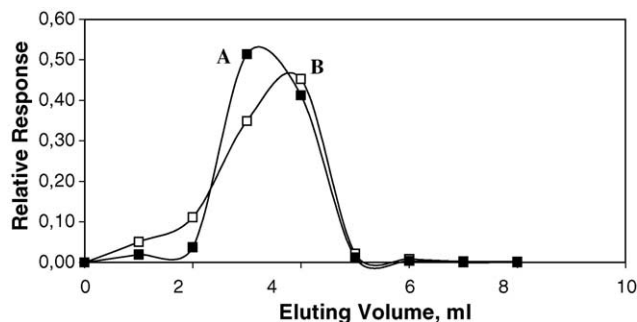
Fig. 4. Elution pattern of MG (A) and LMG (B) from the cation exchange cartridge used in the method. Both analytes were at 25 \mu\text{g}/\text{kg} concentration level.
