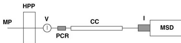
Fig. 2. Manifold for implementation of the method. MP, mobile phase; HPP, high pressure pump; V, injection valve; PCR, oxidative pre-column reactor; CC, chromatographic column; I, APCI interface; MSD, mass detector.
