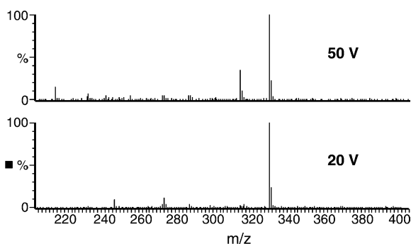
Fig. 5. Mass spectra for MG showing the effect of the cone potential as indicated.
