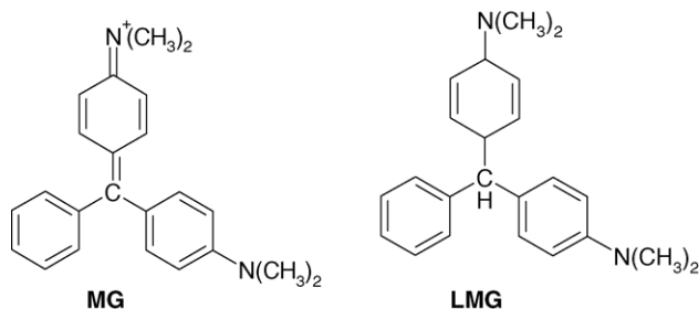
Fig. 1. Chemical structures of malachite green (MG) and leucomalachite green (LMG).
