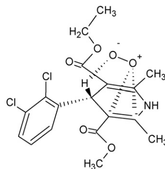
Fig. 5. Proposed encounter complex formed in the first step of the reaction of singlet oxygen with felodipine.
