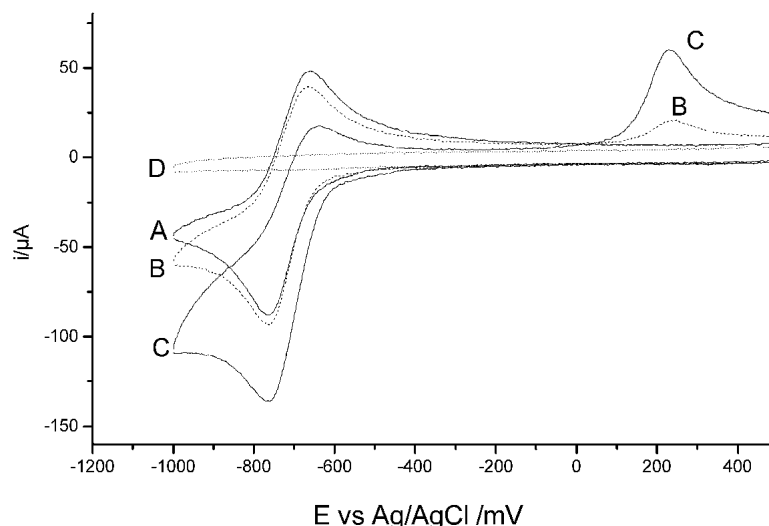
Fig. 4. CVs of the O_2/O_2^{\bullet-} redox couple at the GC electrode in O_2 -saturated DMSO solution in the (A) absence and in the presence of different nifedipine concentrations (B) 3 \times 10^{-3} M and (C) 2 \times 10^{-2} M. Curve (D) shows the CV of 3 mM nifedipine without oxygen (sweep rate, 1 \text{ Vs}^{-1} ).
