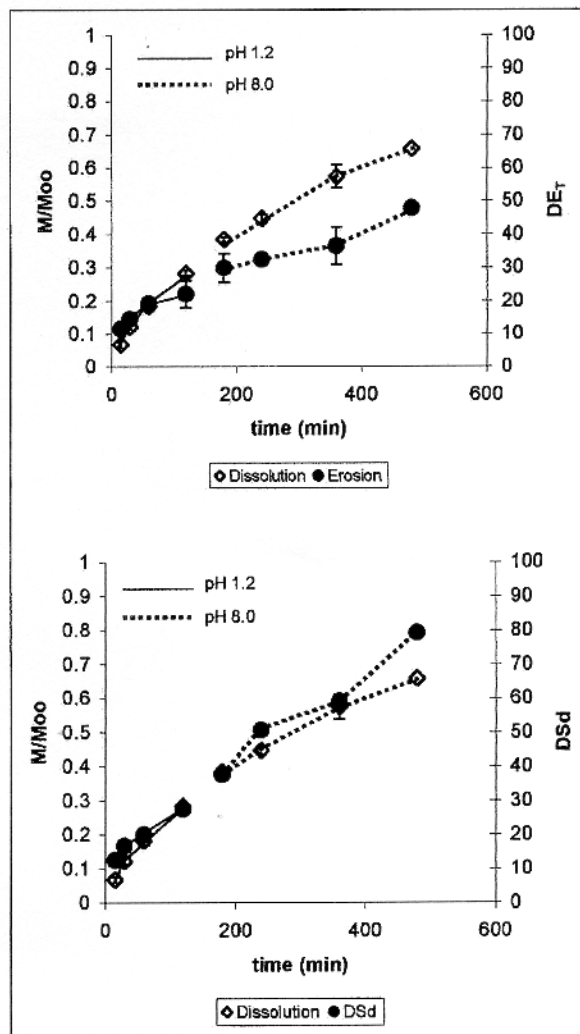
Fig. 7: Correlation between dissolution/erosion and dissolution/swelling behaviour for matrix tablet based on CB-g-A-600 as function of time and pH
