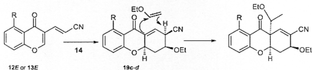
Scheme 5. Plausible mechanism for the formation of 21(c-d) .
