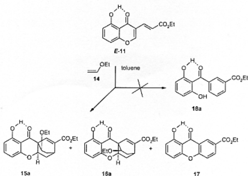
Scheme 2. Domino reaction of ( E )-ethyl 3-(5-hydroxy-4-oxo-4 H -chromen-3-yl)acrylate ( E -11) with ethyl vinyl ether ( 14 )
