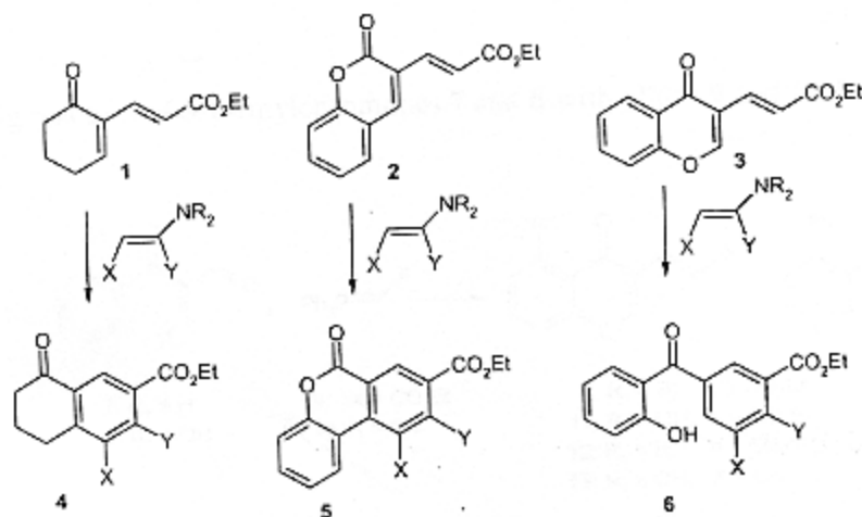
Scheme 1. Reaction of electron-deficient dienes 1-3 with enamines.
