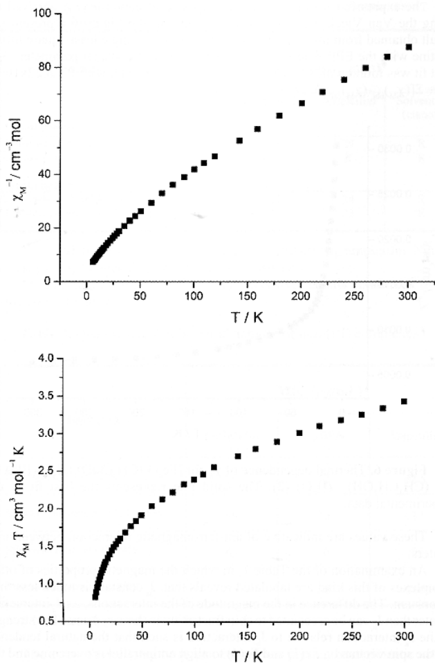
Figure 3. Plot of the temperature dependence of \chi_M^{-1} and \chi_M T for [\text{Fe}_3\text{O}(\text{C}_2\text{H}_3\text{O}_2)_6(\text{C}_2\text{H}_3\text{O}_2)(\text{H}_2\text{O})_2]\cdot\text{Cl}(\text{MeImid})\cdot(\text{H}_2\text{O}) (1)
