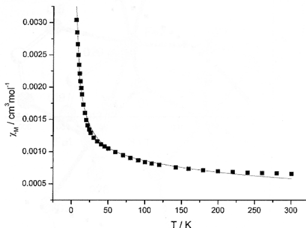
Figure 6. Thermal dependence of \chi_M for [\text{Fe}_4\text{O}_2(\text{CH}_3\text{COO})_7(\text{H}_2\text{O})(\text{BPA})_2]\text{Cl}\cdot(\text{CH}_3\text{CH}_2\text{OH})_2\cdot(\text{H}_2\text{O}) (2). The solid line represents the best fit of the experimental data.
