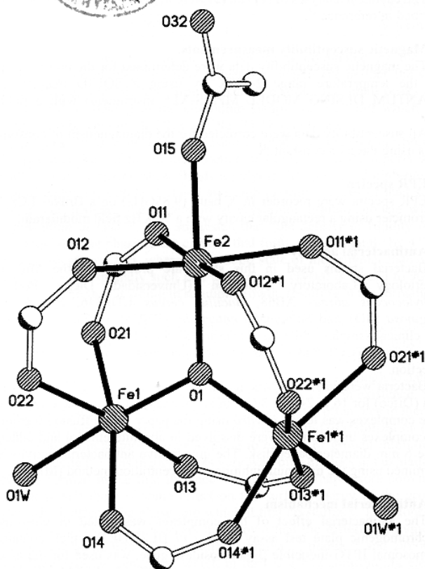
Figure 1. Close view of the trimeric core in ( 1 ), with hydrogen and (some) carbon atoms removed, for clarity.
