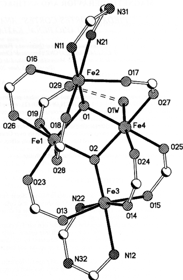
Figure 2. Close view of the tetrameric core in ( 2 ), with hydrogen and (some) carbon atoms removed, for clarity. In double dashed lines, the intramolecular H-bond connecting O1W and acetato 9.
