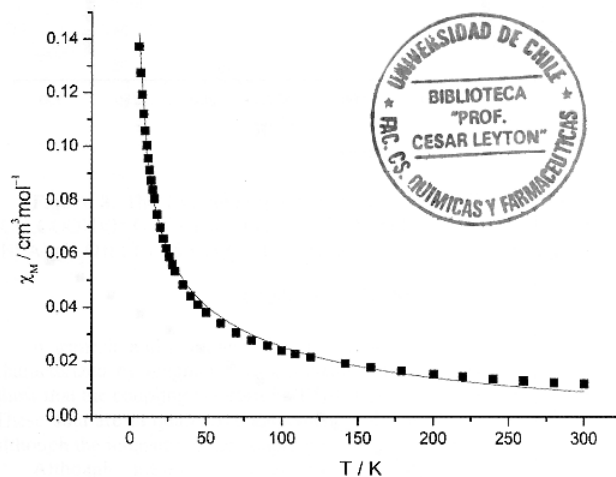
Figure 4. Thermal dependence of \chi_M for [\text{Fe}_3\text{O}(\text{CH}_3\text{COO})_6(\text{CH}_3\text{COO})\text{H}(\text{H}_2\text{O})_2]\cdot\text{Cl}(\text{MeImid})\cdot(\text{H}_2\text{O}) (1). The solid line represents the best fit of the experimental data.
