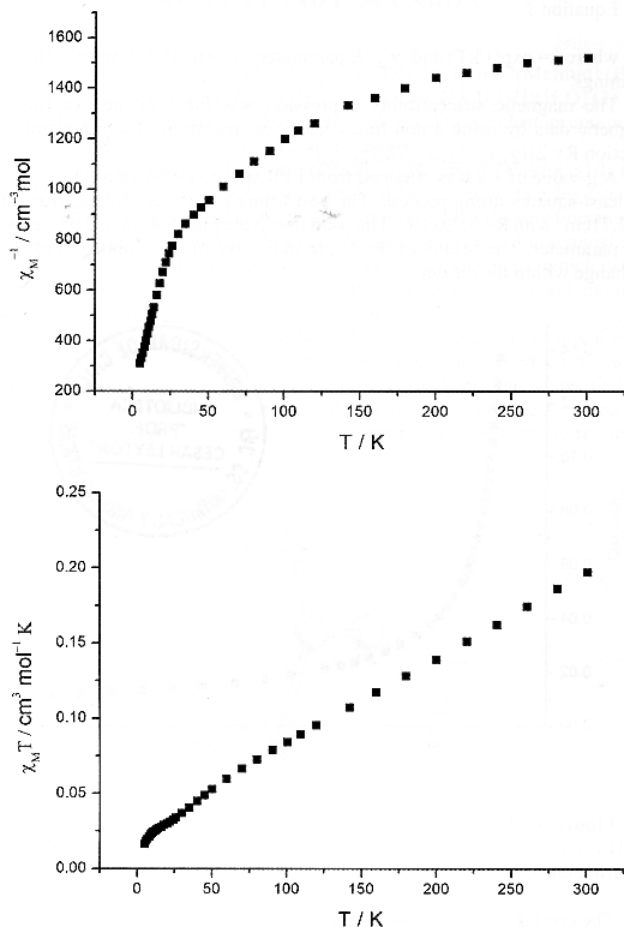
Figure 5. Plot of the temperature dependence of \chi_M^{-1} and \chi_M T for [\text{Fe}_4\text{O}_2(\text{CH}_3\text{COO})_7(\text{H}_2\text{O})(\text{BPA})_2]\text{Cl}\cdot(\text{CH}_3\text{CH}_2\text{OH})_2\cdot(\text{H}_2\text{O}) (2).
