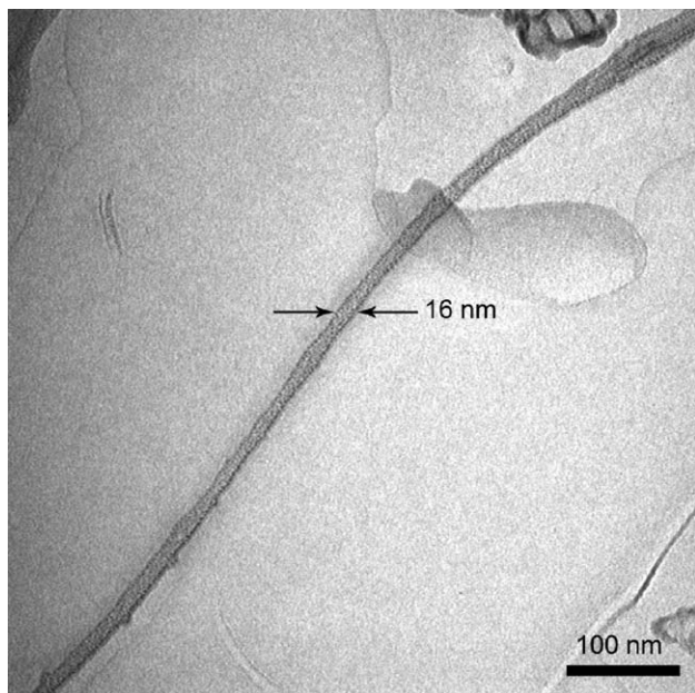
Fig. 6. Transmission electron microscopy image of the replica obtained after freeze-fixation and freeze-drying of a 50 \mu\text{M} aqueous solution of SAP over an uncoated coverslip.
