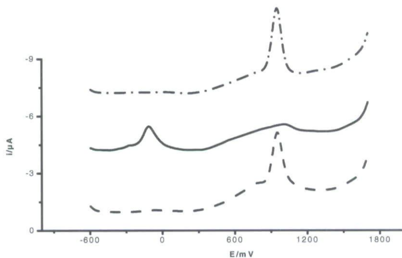
FIGURE 5 Differential pulse voltammograms of 100 \mu\text{M} concentration of 4-M-DHP in acetonitrile. (---) original signal, (—) in the presence of 0.4 mM alcoholic NaOH (— · —) solution with 0.4 mM NaOH in the presence of 0.4 mM \text{HClO}_4 .
