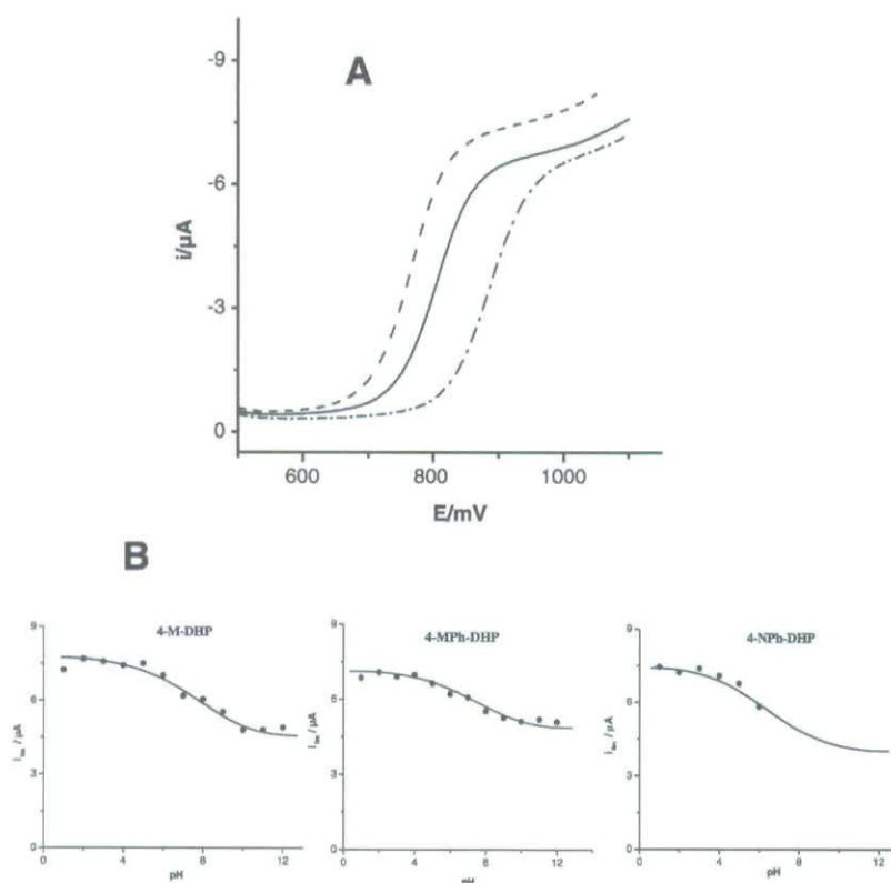
FIGURE 4 (A) Dynamic voltammograms on glassy carbon electrode in protic media at pH 5. (---) 4-M-DHP (—) 4-MPh-DHP (---) 4-NPh-DHP. (B) Dependence of limiting current with pH for a 100 \mu M concentration of 1,4-dihydropyridines in protic media (0.04 M Britton—Robinson buffer + ethanol: 70/30). Rotating rate 5.200 rpm.
