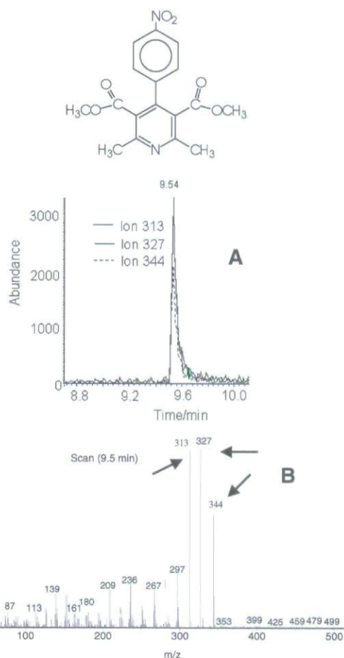
FIGURE 10 Ion chromatogram (A) and mass spectrum (B) corresponding to 4-NPh-DHP derivative after the reaction during 48 hr with ABAP-derived alkyl radicals.
