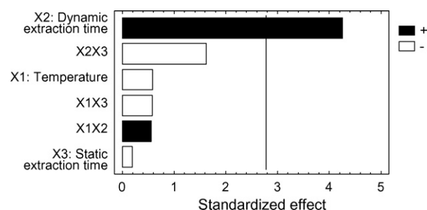
Fig. 1. Standardized Pareto chart.
