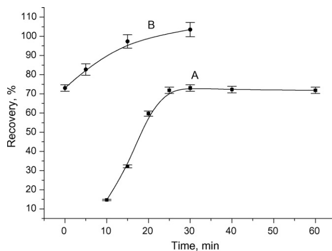
Fig. 2. Recovery of PCBs from biosolid. (A) Effect of dynamic extraction time on recovery. Other conditions: extraction temperature, 50 ^{\circ}\text{C} (without ultrasound assistance). (B) Effect of ultrasound time on recovery. Other conditions: extraction temperature, 50 ^{\circ}\text{C} ; dynamic extraction time, 30 min.
