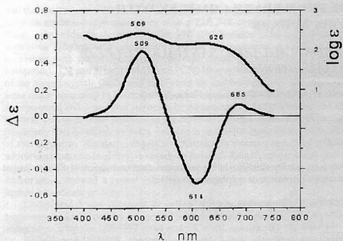
Fig.2 Absorption and circular dichroism spectra of \Delta -hexol synthesized in the presence of D-galactosamine.
