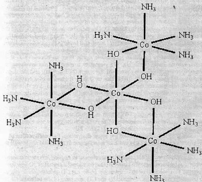
Fig. 1. Structure of \Delta -[Co{(OH) 2 Co(NH 3 ) 4 }] 3 6+ .
