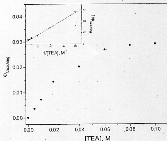
Fig. 5 Effect of TEA concentration on the 4-nitroanisole photobleaching quantum yield in acetonitrile. Insert: relation between inverse of photobleaching quantum yield and inverse of amine concentration according to eqn. (1).
