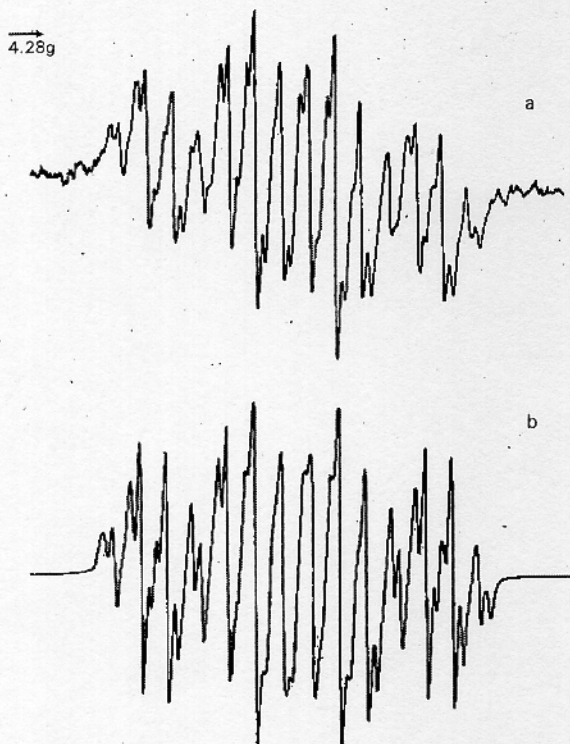
Fig. 3 Effect of nitrosobenzene addition on the EPR spectrum of 4-nitroanisole irradiated in the presence of 0.1 M TEA in acetonitrile at 25 °C. (a) Experimental spectrum; (b) simulated EPR spectrum; linewidth, 0.48 gauss, and Lorentzian/Gaussian ratio of 0.4.
