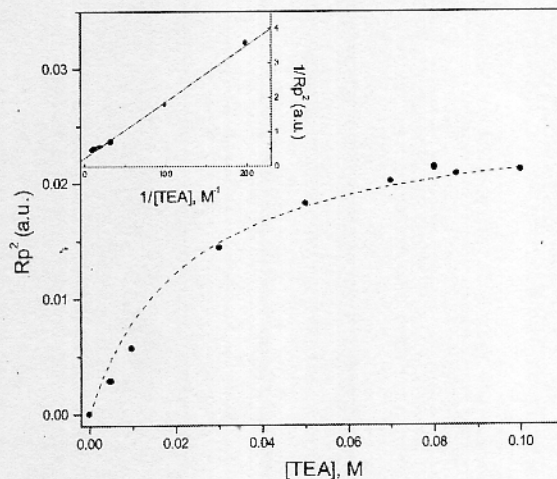
Fig. 6 Effect of the TEA concentration on the methyl methacrylate polymerization rate photoinitiated by 4-nitroanisole in monomer/acetonitrile (1/1). Insert: relation of polymerization rate and amine concentration according to eqn. (3).
