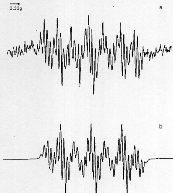
Fig. 4 EPR spectra of 4-nitroacetophenone irradiated in the presence of 0.1 M TEA in acetonitrile at 25 °C. (a) Experimental spectrum; (b) simulated EPR spectrum; linewidth, 0.48 gauss, and Lorentzian/Gaussian ratio of 0.4.
