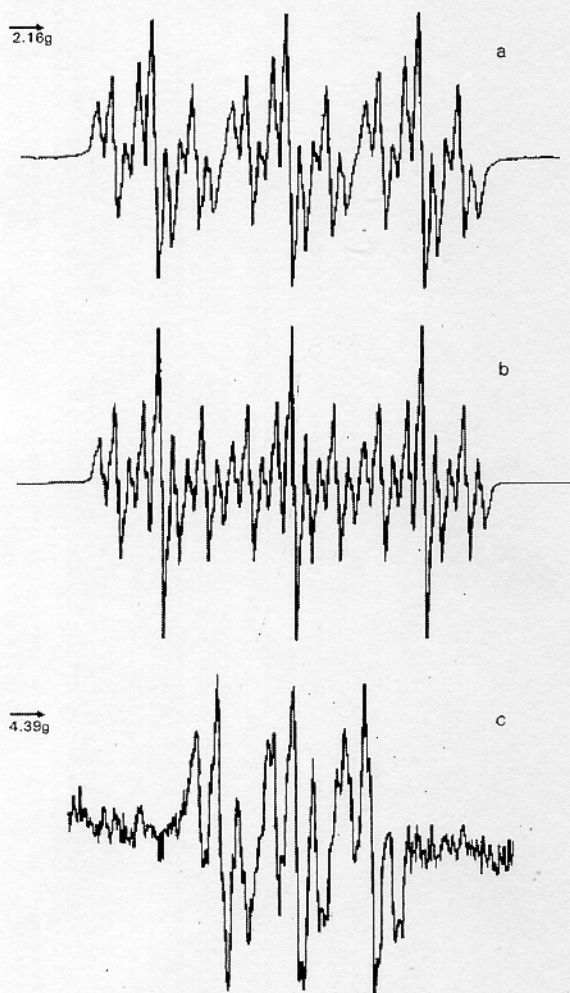
Fig. 2 EPR spectra of the radical anion of 4-nitroanisole in acetonitrile at 25°C, when is generated: (a) by electrochemical reduction; (b) simulated spectrum of the radical anion, with linewidth of 0.4 G and ratio Lorentzian/Gaussian of 0.4; (c) photochemically in the presence of 0.1 M TEA.
