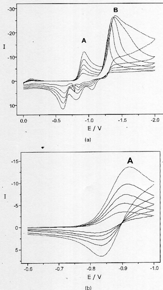
Fig. 1 Cyclic voltammograms of 4-nitroacetophenone at different scan rates, in acetonitrile at 25°C, SCE as reference electrode. Scan rates from the top: 2; 1; 0.5; 0.25; and 0.1 V s -1 . (a) Potential range from 0 to -2.0 V; (b) Potential range from -0.6 to -1.0 V.
