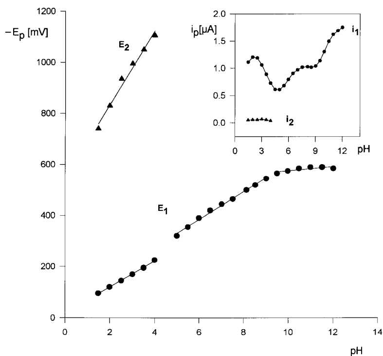
Fig. 3. Differential pulse peak potential and peak current (inset) dependence of 0.1 mM flutamide solution with pH.
