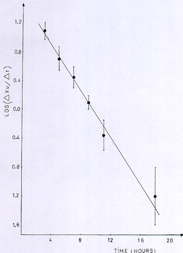
Fig. 2 Mean excretion rate vs time profiles of dibekacin in 10 normal subjects following a 2 \text{ mg} \cdot \text{kg}^{-1} i.v. bolus injection.
