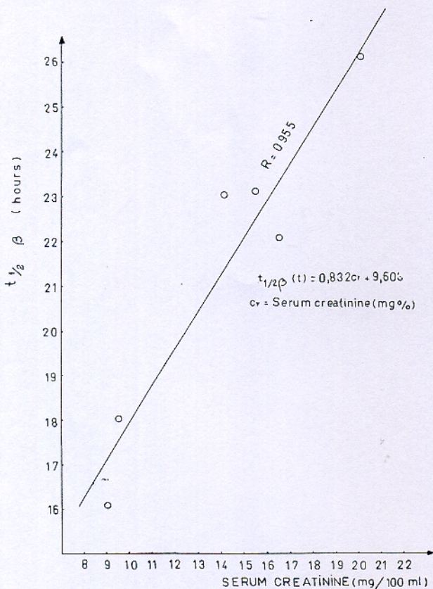
Fig. 4 Relationship between serum creatinine concentration and the beta half-life of dibekacin.
