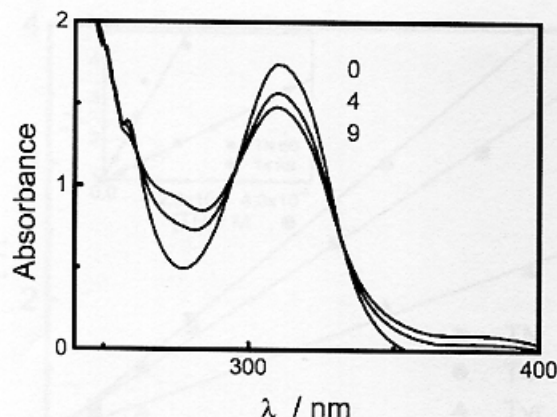
Figure 1. Spectral evolution of I 2 Tyr sensitized by perinaphthenone, on visible light irradiation, in water-KOH 10 mM. Numbers on the spectra represent irradiation time (minutes).
