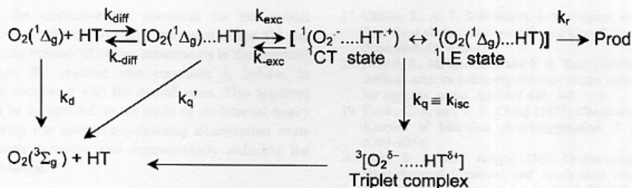
Scheme 3. Modified Scheme 2.
