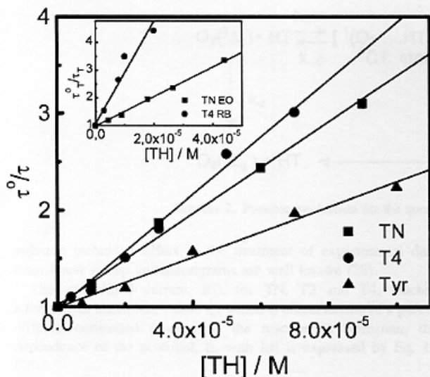
Figure 2. Stern-Volmer plots for the quenching of O_2(^1\Delta_g) luminescence by TN, T4 and Tyr. Inset: Stern-Volmer plots for the quenching of ^3RB^* by T4 and ^3EO^* by TN (Argon-saturated solutions).
