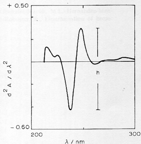
Fig. 3. Second-derivative spectrum of 10 \mu\text{g ml}^{-1} bromazepam vs water. \Delta\lambda = 5 ; h = 0.723 .
