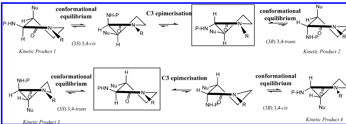
FIGURE 2. Thermodynamic control of the relative stereochemistry of C3 and C4 of 3,4-disubstituted piperidones 8 .
