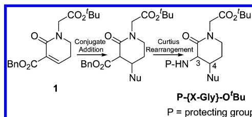
FIGURE 1. Synthesis of X-Gly pseudopeptides.
