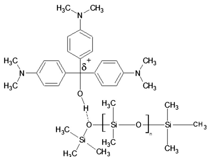
Fig. 3. Interaction by hydrogen bond between carbinol-CV and PDMS.
