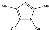
Scheme 1 The 3,5-dimethylpyrazolate ( 3,5\text{-Me}_2\text{pz}^- ) ligand connecting two copper atoms, as found in complexes 1 and 2 .
