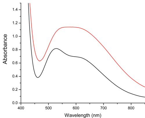
Fig. 6 Absorption spectra of 1 (red) and 2 in \text{CHCl}_3 .
