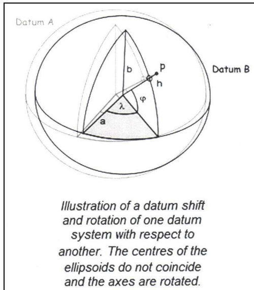
Figure 2. Same point (p), different Datum, different coordinates.
