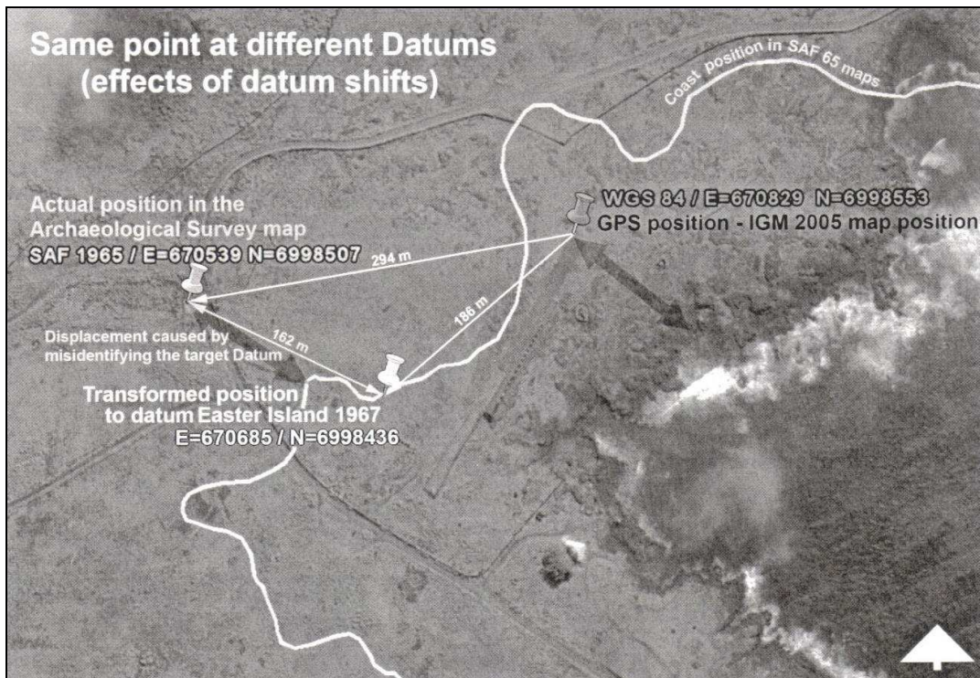
Figure 3. Displacements determined at Ahu Tongariki between SAF 65 charts, Datum WGS 84 georeferenced image and transformed position from GPS readings to Datum Easter Island 1967.
