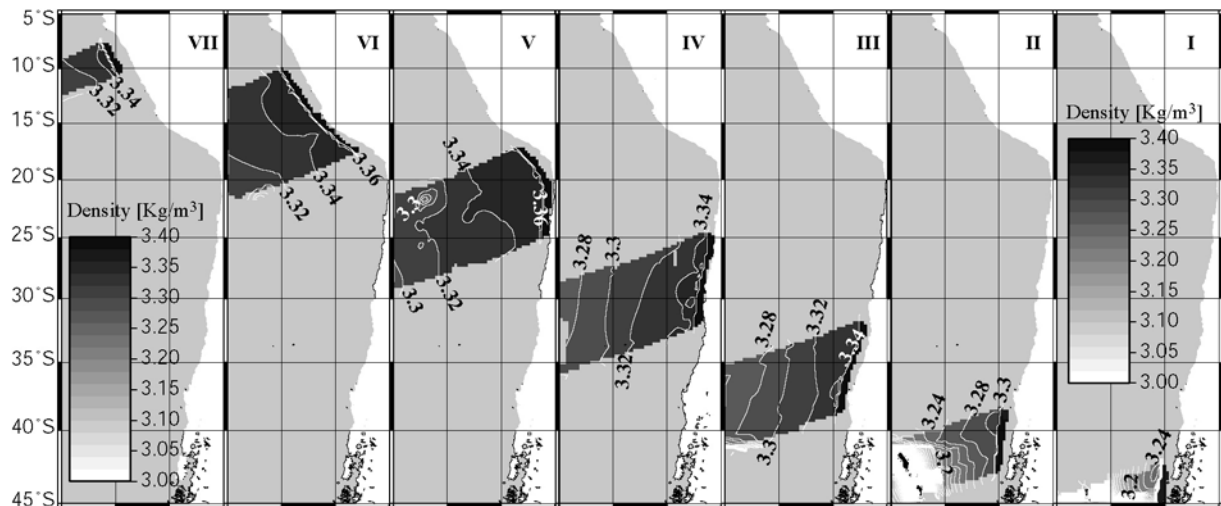
Fig. 4.8. Density structure of the Nazca plate lithospheric mantle. Panels show the results of the procedure discussed in the text and appendix B for each of the seven modelled segments forming the oceanic plate.
