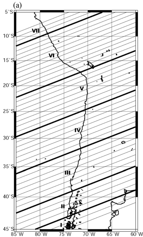
Fig. 4.2. (a) Distribution of the 43 vertical cross-section from which the three-dimensional density structure of the model is triangulated. Thick lines coincide with fracture zones from Plate 1a and correspond to cross-sections dividing the density structure of the oceanic plate and subducted slab in seven segments that are labelled with roman numbers I to VII. (b) One of the vertical cross-sections showing the downward extension of the model till 410 km and its general density structure. 4-times vertical exaggeration. Triangles represent volcanoes. Columns along figure's extreme labelled RM represent the reference density model with values in \text{Mg/m}^3 . Abbreviations of bodies and their densities are defined in Table 1. See text for description.
