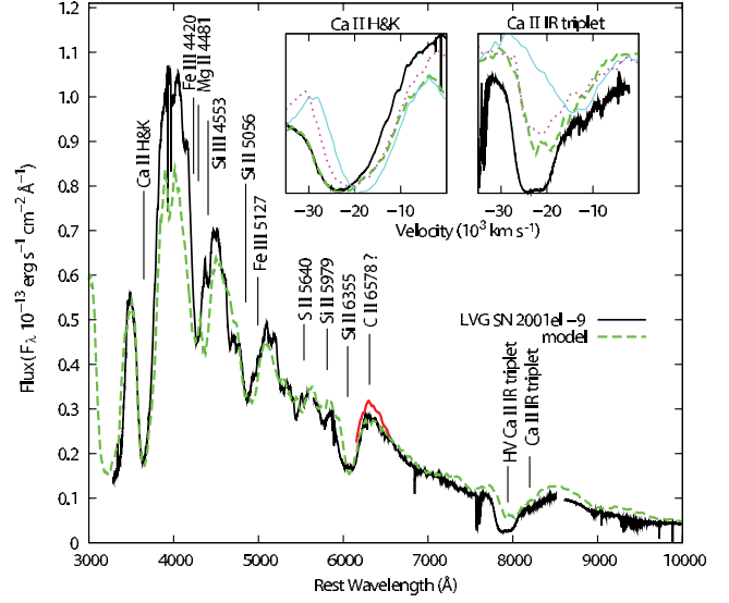
FIG. 5.— Observed spectrum of the LVG SN 2001el at day -9 (black solid lines) and a model with W7-CSM density/abundance structure (green dashed lines). The red solid line shows the profile without C in the ejecta. As in Fig. 1, the left inset shows Ca II H and K, the right inset Ca II IR. The W7-CSM spectrum is compared to W7 (thin cyan lines) and DD (red dotted lines) models, both with homogeneous abundance and without CSM interaction.
