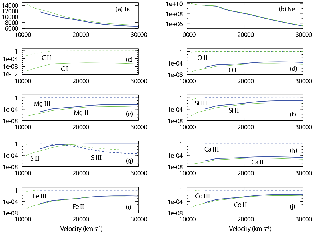
FIG. 9.— Radial distribution of (a) radiation temperature (K), (b) number density of electrons (cm -3 ), and (c–j) ionization fraction of each element. Blue lines show the values for a HVG SN (2002bo) and green lines for a LVG SN (2001el). The two dominant ionization states are shown inside each panel; solid lines represent the lower state (e.g., C I, O I, Mg II). In (c), no blue lines appear, because C is not included in the models of HVG SNe.
