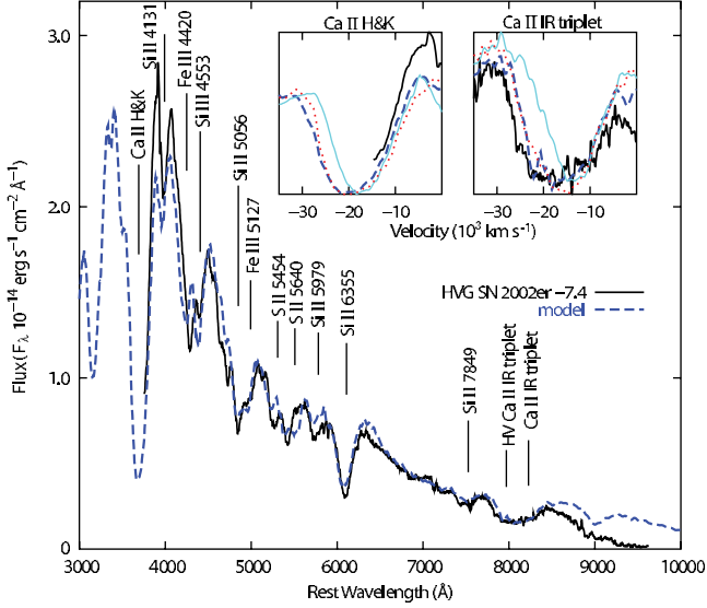
FIG. 4.— Observed spectrum of the HVG SN 2002er at day -7.4 (black solid lines) and a model with W7-CSM density/abundance structure (blue dashed lines). As in Fig. 1, the left inset shows Ca II H and K, the right inset Ca II IR. The W7-CSM spectrum is compared to W7 (thin cyan lines) and DD (red dotted lines) models, both with homogeneous abundance and without CSM interaction.
