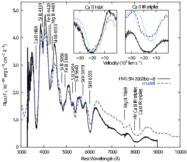
FIG. 1.— Observed spectrum of the HVG SN 2002bo at day -8 (black solid lines) and a model with W7-CSM density/abundance structure (blue dashed lines). The left inset shows the Ca II H and K feature (mean \lambda \sim 3950 ), the right inset the Ca II IR feature (mean \lambda \sim 8567 ). The W7-CSM spectrum is compared to W7/homogeneous abundance (thin cyan lines) and DD (red dotted lines) models, both without CSM interaction. In both insets, the wavelength scale is replaced by the corresponding Doppler velocities.
