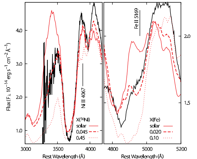
FIG. 2.— SN 2002bo: Observed spectrum around 3500 \text{ \AA} (left) and 4900 \text{ \AA} (right) compared with synthetic profiles for different metal abundances.
