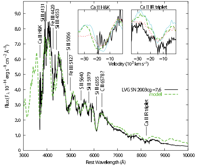
FIG. 6.—Observed spectrum of the LVG SN 2003cg at day -7.6 ( black solid lines ) and a model with W7-CSM density/abundance structure ( green dashed lines ). This model uses stratification with three abundance zones (§ 3.5.3). As in Fig. 1, the left inset shows Ca II H and K, the right inset Ca II IR. The W7-CSM spectrum is compared to W7 ( thin cyan lines ) and DD ( red dotted lines ) models, both with homogeneous abundance and without CSM interaction.
