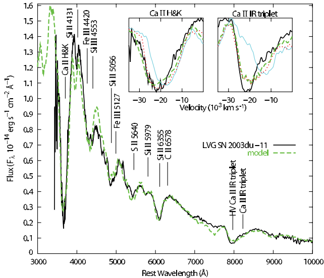
FIG. 7.— Observed spectrum of the LVG SN 2003du at day -11 (black solid lines) and a model with W7-CSM density/abundance structure (green dashed lines). As in Fig. 1, the left inset shows Ca II H and K, the right inset Ca II IR. The W7-CSM spectrum is compared to W7 (thin cyan lines) and DD (red dotted lines) models, both with homogeneous abundance and without CSM interaction.
