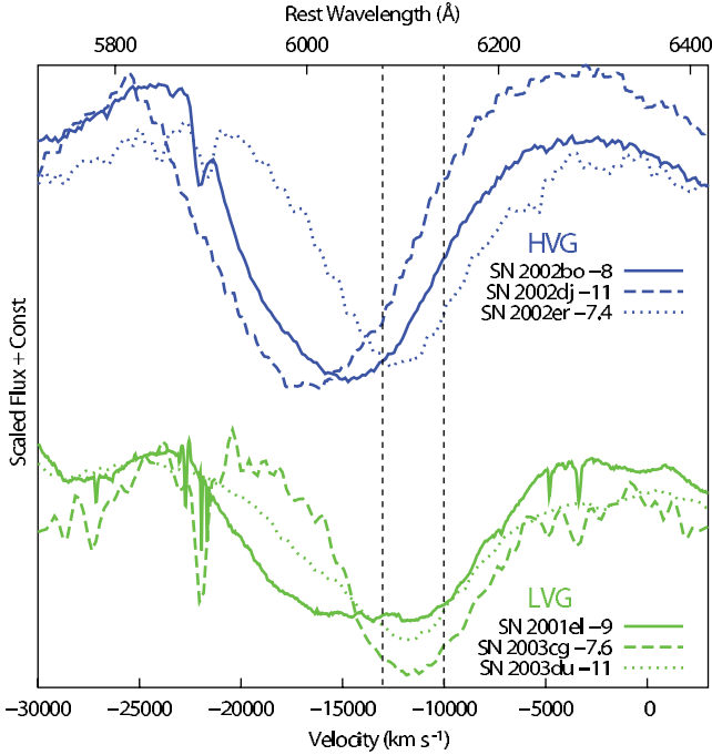
FIG. 8.— Observed Si II \lambda 6355 features of three HVG SNe Ia (upper blue lines) and three LVG SNe Ia (lower green lines). Velocities and shapes of the blue wing differ among the objects. They range from 15,000 km to 25,000 km s -1 irrespective of the SN group (HVG, § 4.1, or LVG, § 4.2). The black dashed lines correspond to Doppler velocities of v = 10,000 and 13,000 km s -1 , which are the typical photospheric velocities of LVGs and HVGs, respectively.
