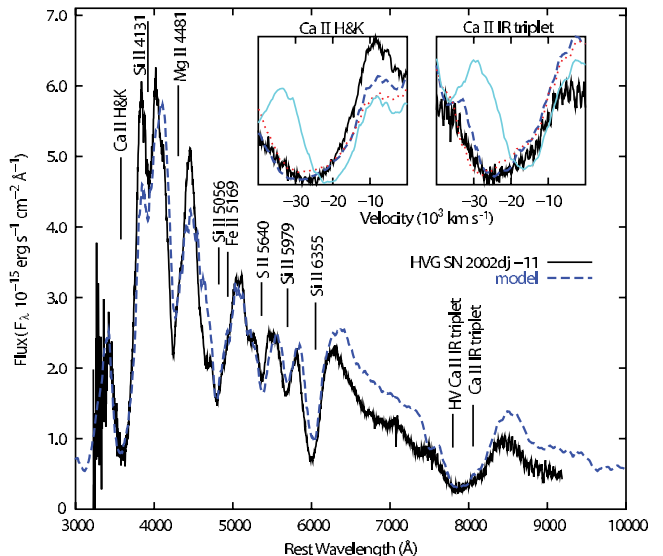
FIG. 3.— Observed spectrum of the HVG SN 2002dj at day -11 (black solid lines) and a model with W7-CSM density/abundance structure (blue dashed lines). As in Fig. 1, the insets show \text{Ca II H} and \text{K} (left) and \text{Ca II IR} (right). The W7-CSM spectrum is compared to W7 (thin cyan lines) and DD (red dotted lines) models, both with homogeneous abundance and without CSM interaction.
