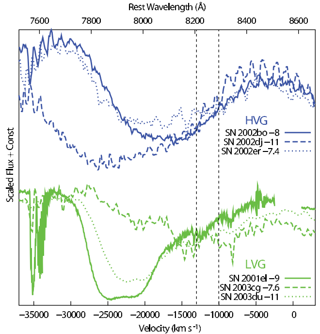
FIG. 10.—Ca II IR triplet profiles (a mean wavelength of 8567 \text{ \AA} is assumed) of three HVG SNe Ia ( upper blue lines ) and three LVG SNe Ia ( lower green lines ). In LVG SNe (SNe 2001el and 2003du in our sample and SN 2003kf in Mazzali et al. 2005b), HVFs tend to be detached, which is likely the consequence of the high photospheric temperature and the low photospheric velocity (see § 4.5). On the other hand, the strength of the high-velocity absorption seems to be random (Tanaka et al. 2006). The dashed black vertical lines correspond to Doppler velocities of v = 10,000 and 13,000 \text{ km s}^{-1} , which are the typical photospheric velocities of LVGs and HVGs, respectively.
