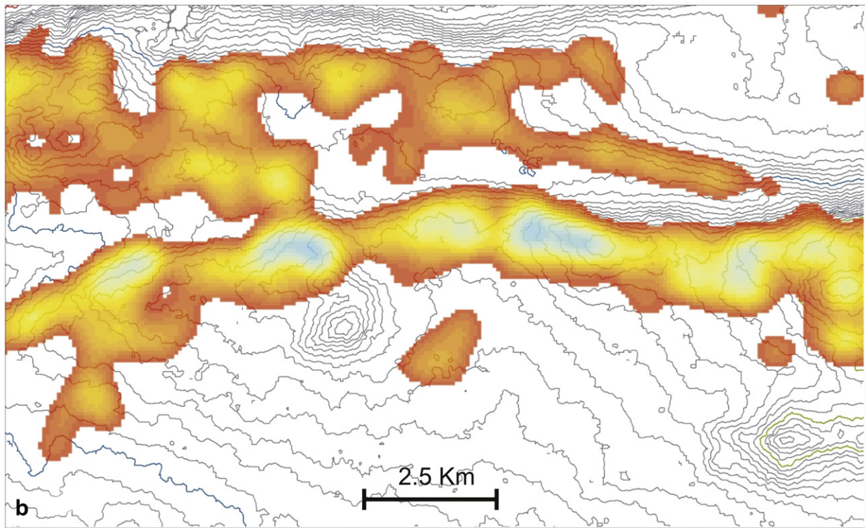
Fig. 8. (a) Distribution of fracture centroids and topography of the reverse-fault scarp; 50 m topographic contour interval. (b) Details of fracture centroid density. Note that high-density clusters; violet and blue colours are not exposed on the uppermost part of the topography; 15 m topographic contours.
