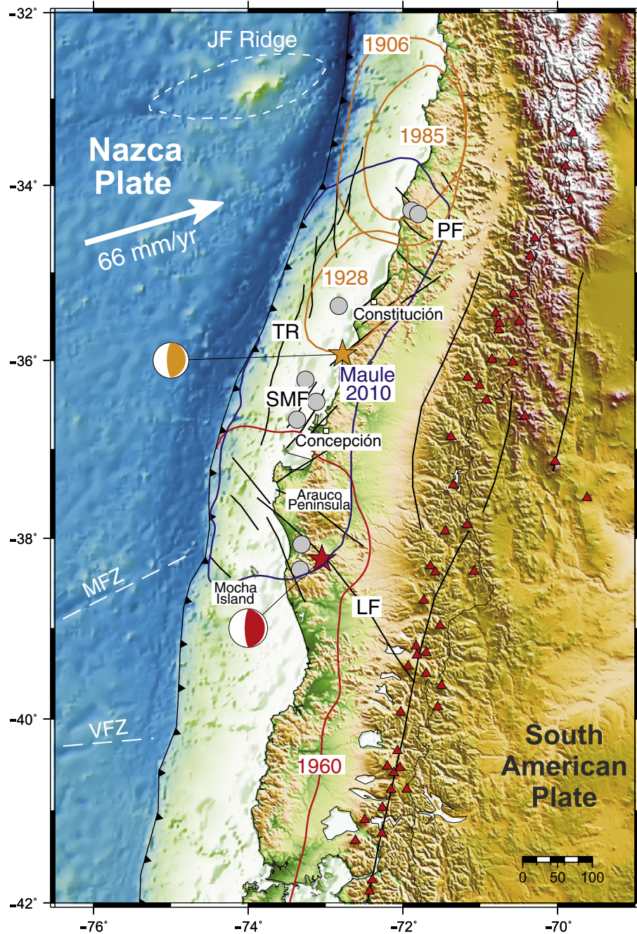
Fig. 1. Seismotectonic setting of the South-Central Chile megathrust. The rupture zone ( >1 m) and fault plane solutions of the 2010 Maule and 1960 Valdivia megathrust earthquakes are shown in blue and red, respectively. Orange lines depict rupture zones of the 1906, 1928 and 1985 events. Gray circles are epicentral locations of largest aftershocks ( M_w > 6.5 ). Black lines denote major upper plate faults consisting of the Thrust Ridge (TR), Santa María Fault (SMF), Llanhue Fault (LF) and Pichilemu Fault (PF). White dashed lines represent the main oceanic features of the Nazca Plate in the study area, which consist of the Juan Fernández Ridge (JF Ridge), and Mocha (MFZ) and Valdivia (VFZ) fracture zones. Red triangles indicate active volcanoes. (For interpretation of the references to color in this figure legend, the reader is referred to the web version of this article.)
