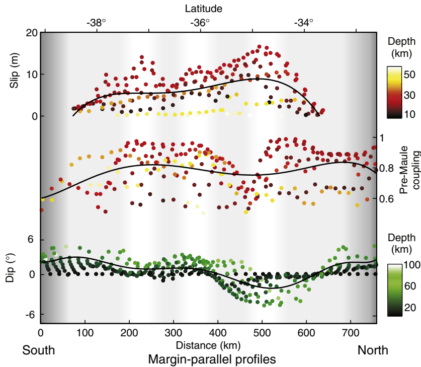
Fig. 9. Margin-parallel profiles of coseismic slip, interseismic locking degree and margin-parallel dip of the slab. Points are colored by their depth. (For interpretation of the references to color in this figure legend, the reader is referred to the web version of this article.)
