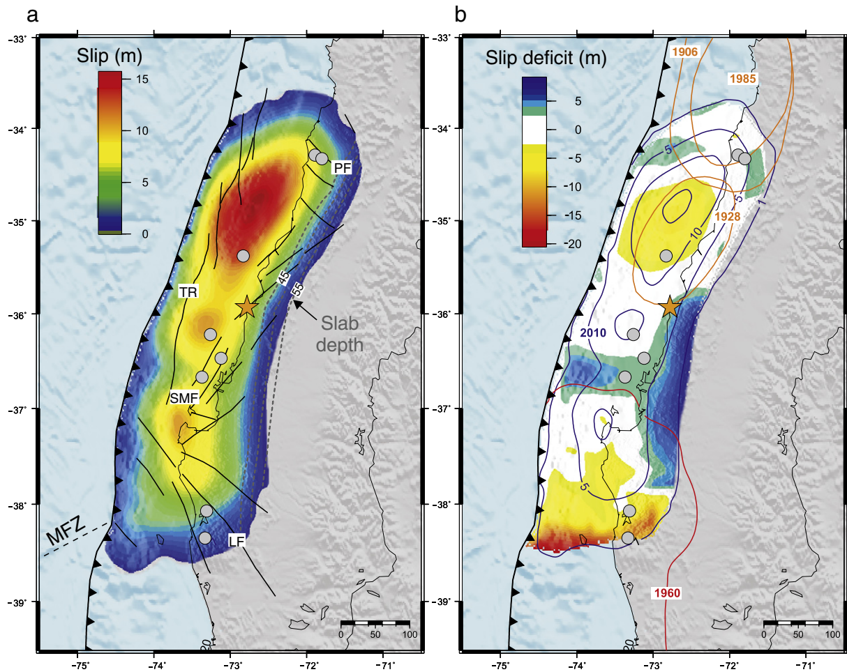
Fig. 6. a) Preferred coseismic slip model for the 2010 Maule earthquake. Black lines denote the Thrust Ridge (TR), Santa María Fault (SMF), Lanahue Fault (LF) and Pichilemu Fault (PF). Gray circles are epicentral locations of largest aftershocks ( M_w > 6.5 ). Dashed gray lines at the down-dip of the rupture depict the slab depth (5-m contours). b) Slip deficit estimation along the rupture area of the Maule earthquake. Shown are the rupture zones of the 1906, 1928, 1985, 1960 and 2010 earthquakes.
