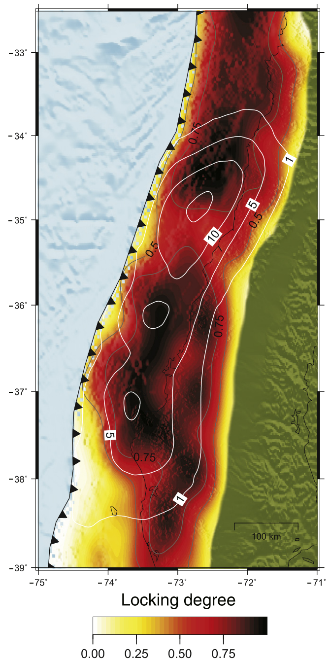
Fig. 7. Coseismic slip distribution, shown with 5-m slip contours, overlain on the locking degree distribution, which is also shown by brown 0.25-degree contours (Moreno et al., 2010).
