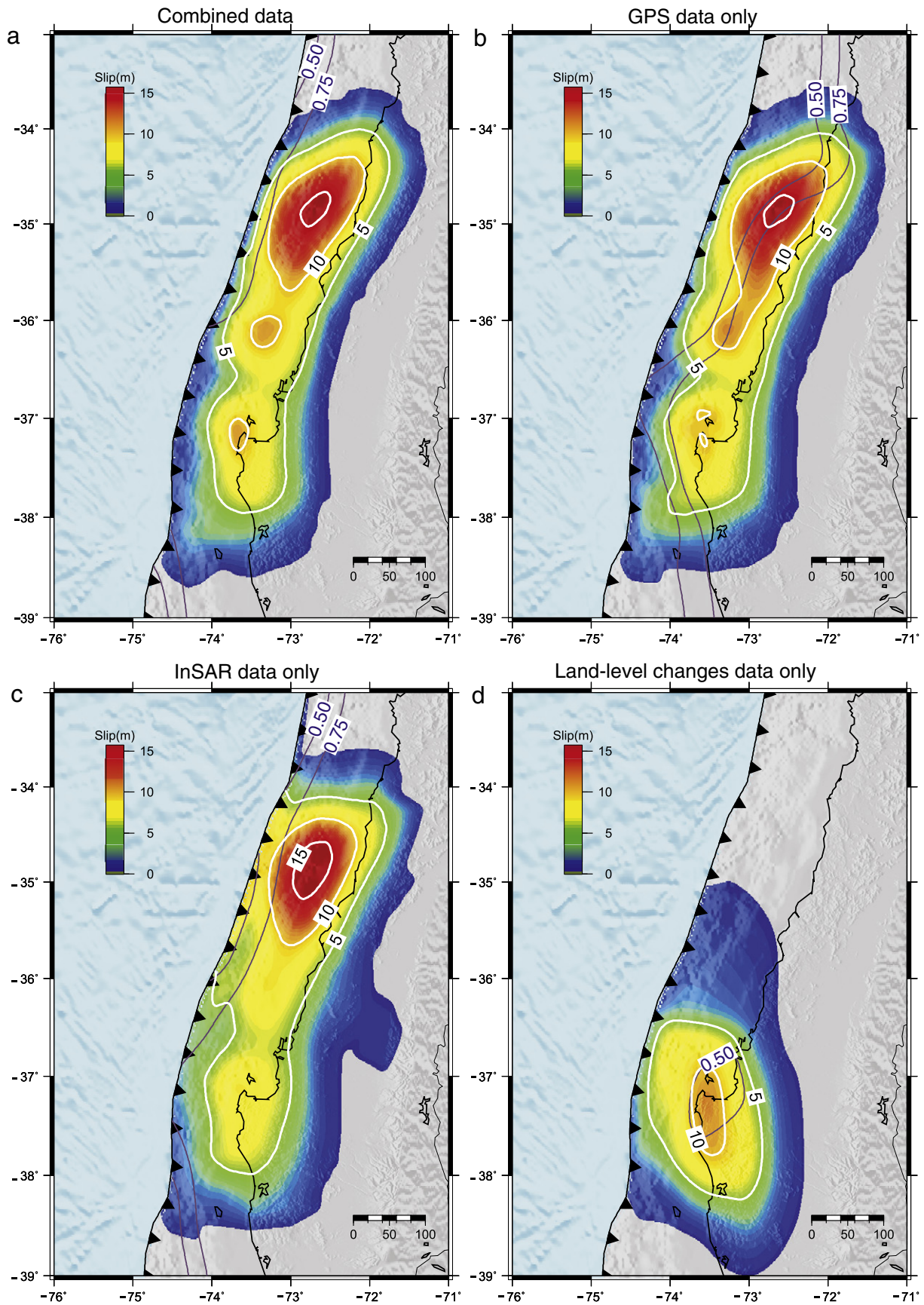
Fig. 4. Total coseismic slip obtained by using different data sets. a) Joint inversion of GPS, InSAR and land-level changes. b) Slip model from inversion of GPS data alone. c) Slip model from inversion of InSAR data alone. d) Slip model from inversion of land-level changes alone. Gray contours show the resolution for each inversion.
