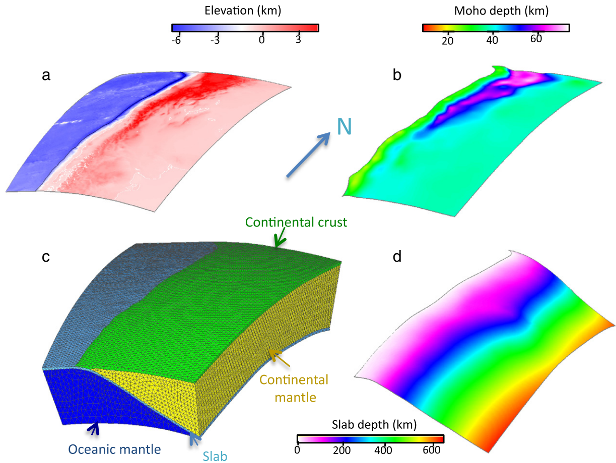
Fig. 3. 3-D model configuration. The FE-model includes topography and bathymetry, as well as a precise geometry of the slab and continental Moho, which were derived from combining available geophysical information. a) Topography and bathymetry introduced in the FE-model. b) Continental Moho discontinuity along the Chile subduction margin. c) Mesh structure of our FE-model. d) Upper surface of the plate interface used in this study.
