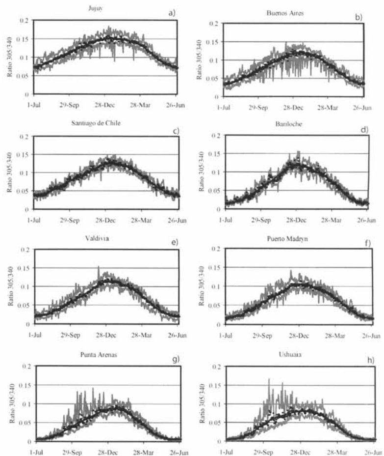
Figure 6. Ratio channel 305/channel 340. Historical maximum (upper full grey line), minimum (lower full grey line), mean (dotted line) and annual cycle (full black line), calculated from maximum daily irradiance values for the period 1995–2002, except for Bariloche, which includes values from 1998–2002.
