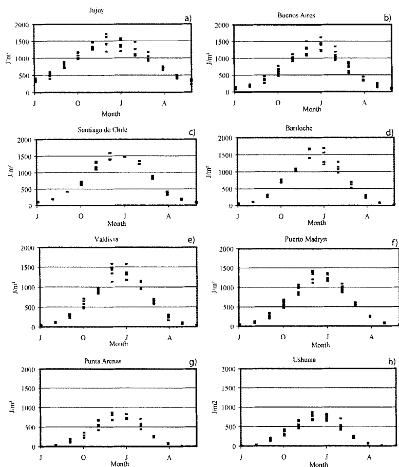
Figure 5. Monthly average of the daily integrated irradiance for the 305 nm channel.
