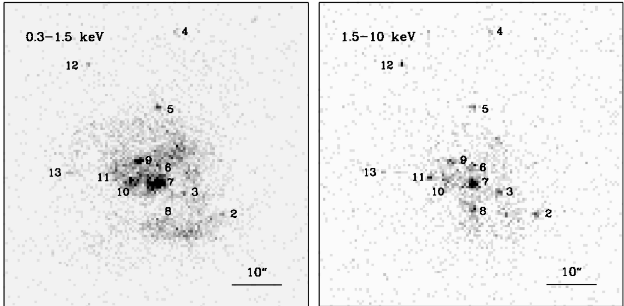
Figure 1. Chandra images of NGC 3256 in the 0.3–1.5 keV (left) and 1.5–10 keV (right) energy ranges. The images extend \sim 60 arcsec on each side. North is at the top and East is on the left. Discrete sources are labelled by increasing order of right ascension. Sources 1 and 14 are not included in the figure (see Table 1 for celestial coordinates).
