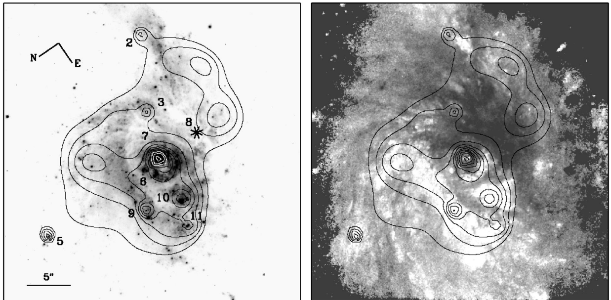
Figure 10. X-ray isocontours overlaid onto optical HST PC2 images of the central region in NGC 3256. A broad-band F814W ( \sim I ) image is shown in the left panel and a colour F450W-F814W ( \sim B - I ) image is shown at the right (darker corresponds to redder colours – for a colour version see fig. 2 in Zepf et al. 1999). Both images have the same size and (non-standard) orientation. Compact sources are labelled and the position of the southern nucleus is marked with an asterisk in the top image.
