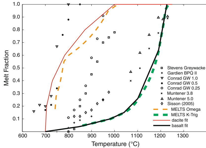
Fig. 8 Summary of melt fraction–temperature relationships observed in various experimental studies and those ultimately used in thermal models. Sources for experimental data: squares are graywacke from Stevens et al. (1997); plus symbols are graywacke from Gardien et al. (1995); upside-down triangles, stars, and circles are graywacke with varying water contents from Conrad et al. (1988); cross-symbols and upward-facing triangles are basalts with varying water contents from Muntener et al. (2001); and diamonds are basalt (87S35A) from Sisson et al. (2005). The thin dashed (orange) curve is a MELTS simulation using the \Omega dacite bulk rock composition, NNO, 2 kbars, and 3 wt% H 2 O; while the shape of this curve did not change
