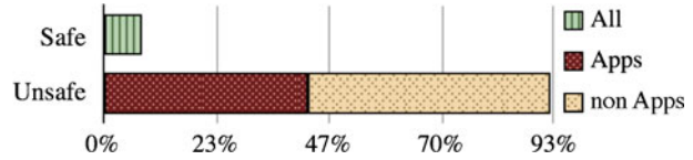
Fig. 10 Safe/unsafe usages of superclass updates
