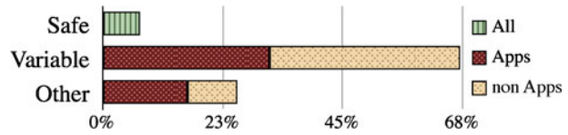
Fig. 8 Safe/unsafe usages of message sending
