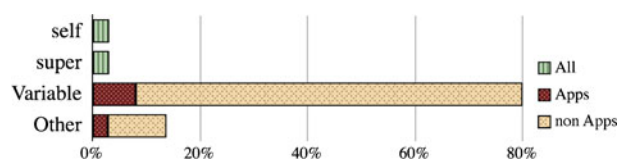
Fig. 9 Safe/unsafe usages of class deletion
