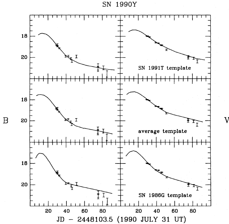
FIG. 8. The B and V light curves of SN 1990Y are compared to the slow-decliner SN 1991T template light curves (top panel), to the SNe Ia average templates calculated by Leibundgut (1988) (middle panel), and to the fast-decliner SN 1986G templates (bottom panel). All of the templates were properly modified by the K -terms and the time dilatation calculated by Hamuy et al. (1993).
