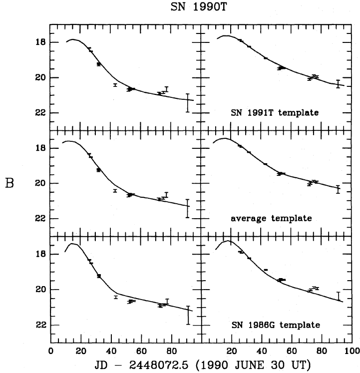
FIG. 6. The B and V light curves of SN 1990T are compared to the slow-declining SN 1991T template light curves (top panel), to the SNe Ia average templates calculated by Leibundgut (1988) (middle panel), and to the fast-decliner SN 1986G templates (bottom panel). All of the templates were properly modified by the K -terms and the time dilatation calculated by Hamuy et al. (1993).
