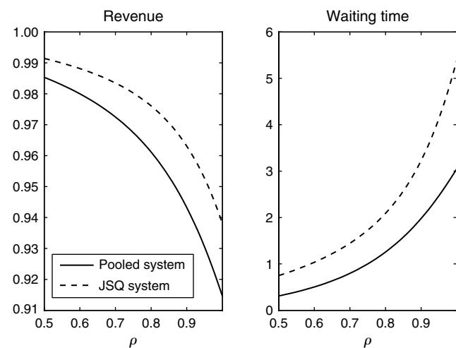
Figure 8 Comparison Between the Split JSQ and Pooled Systems
