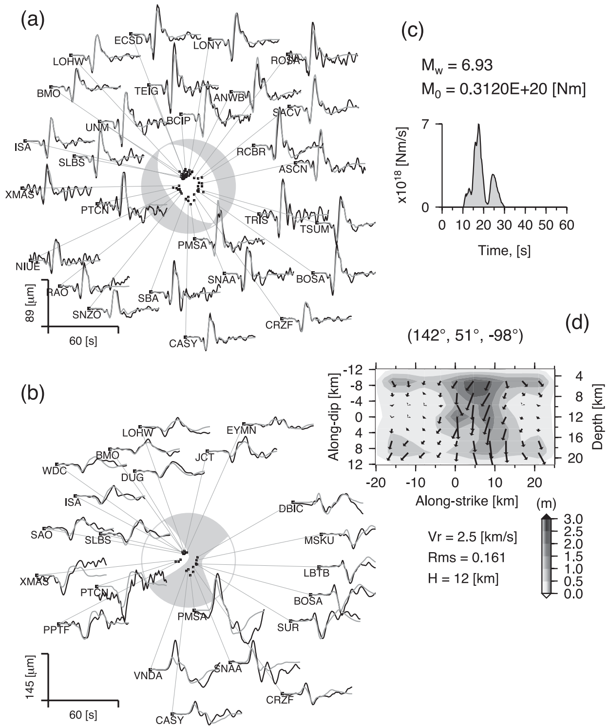
Figure 7. Telesismic finite source model for Event 1, obtained by jointly inverting P and SH waveforms. Comparison of observed (black line) and synthetic (grey line) telesismic waveforms for (a) P and (b) SH waves. (c) Final slip distribution, moment rate source–time function, and corresponding focal mechanism. The rupture speed was fixed to V_r = 2.5 \text{ km s}^{-1} , and the (0, 0) point along-dip and along-strike directions corresponds to the nucleation location. Arrows represent the slip direction on the fault scaled to slip amplitude.
