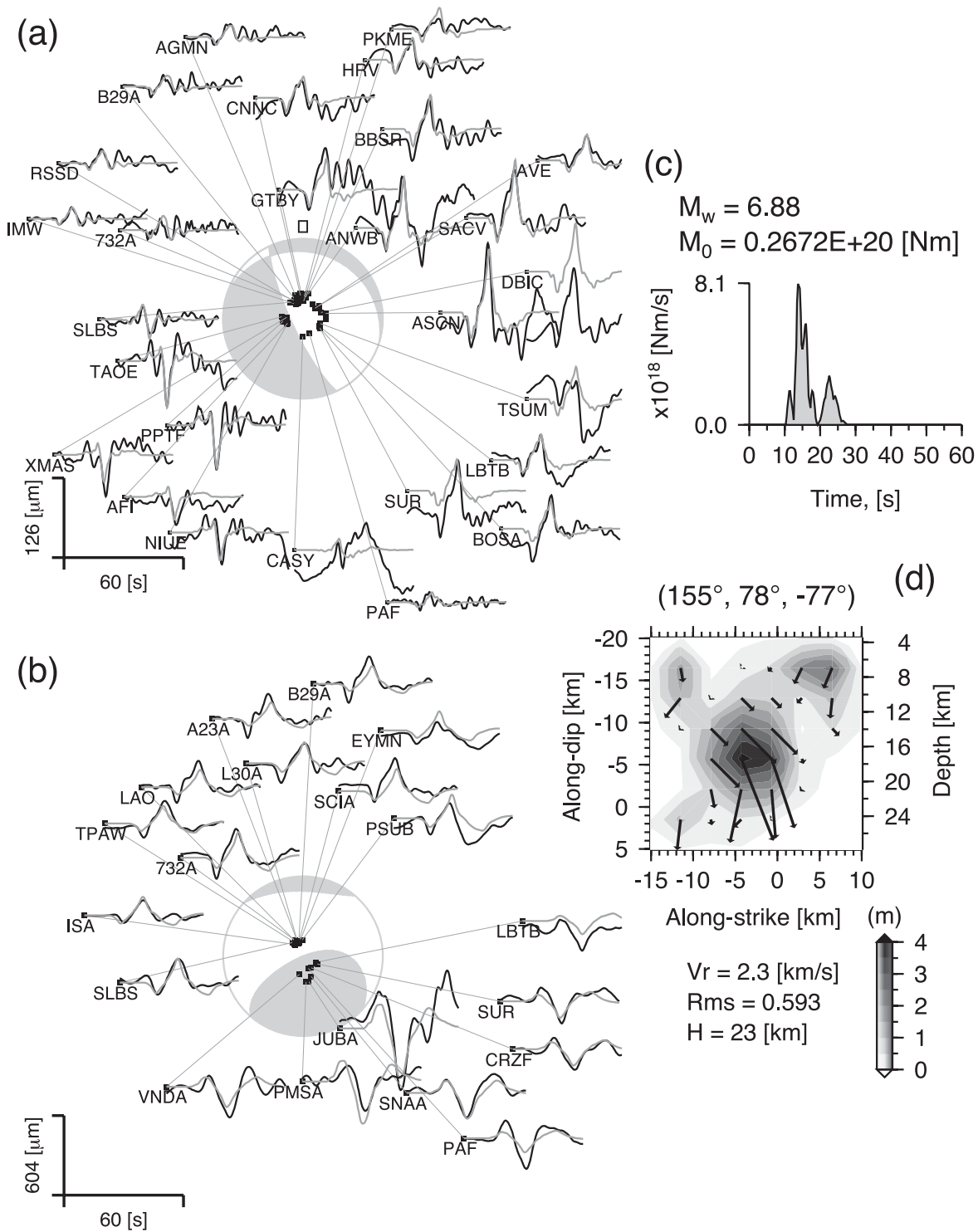
Figure 8. Teleseismic finite source model for Event 2. See Fig. 7 caption for details.
