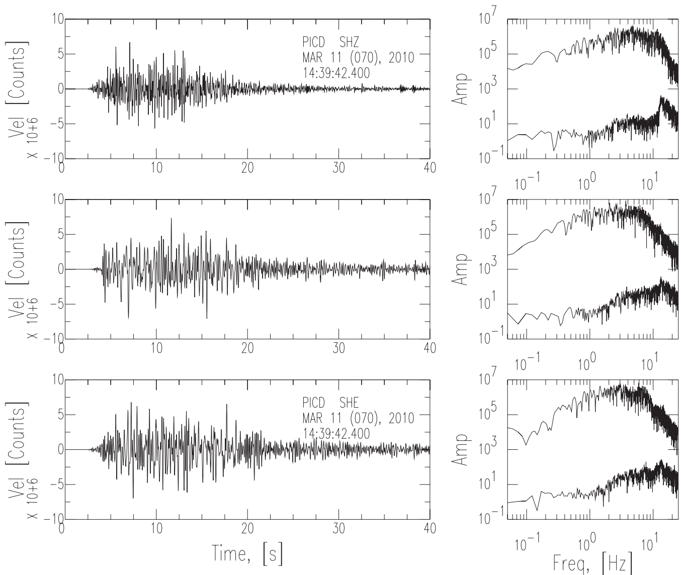
Figure 2. Short-period recording of Event 1 at PICD. Left-hand panel: ground velocity (vertical, north and east components), and right-hand panel: comparison of signal and noise Fourier spectrum amplitudes.
