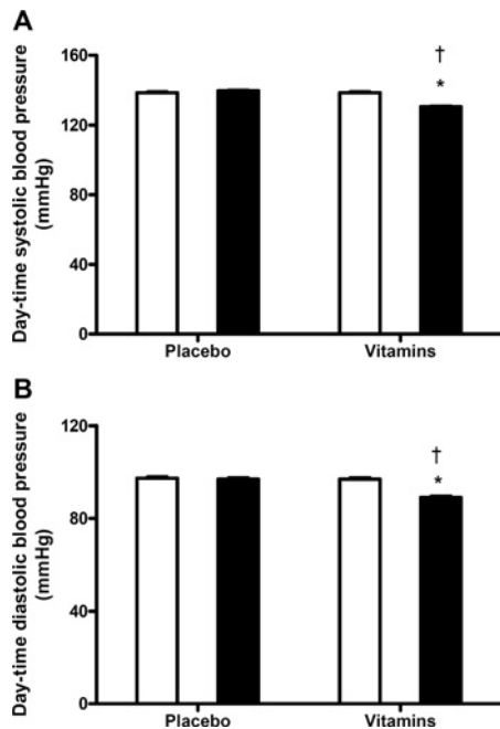
Figure 1 Daytime SBP (A) and DBP (B) in patients with EH before (open bars) and after (closed bars) treatment with either vitamins C + E or placebo
