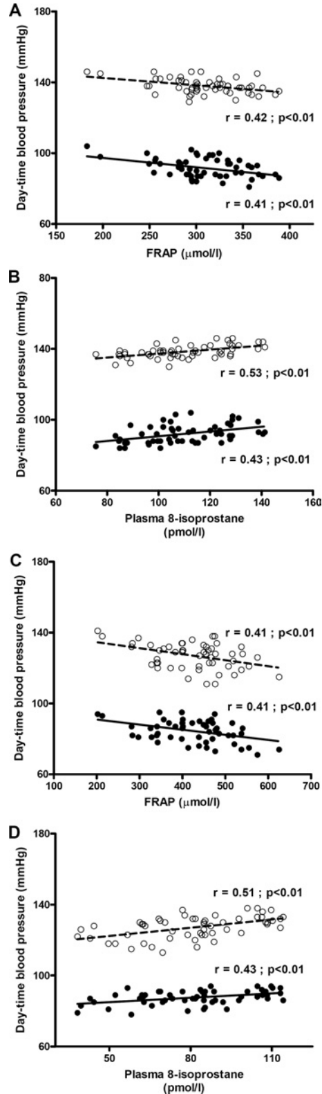
Figure 4 Pearson correlation of SBP (○) and DBP (●) with plasma antioxidant capacity (FRAP) and plasma 8-isoprostane levels in patients with EH following treatment with either placebo (A and B) or vitamins C + E (C and D)
