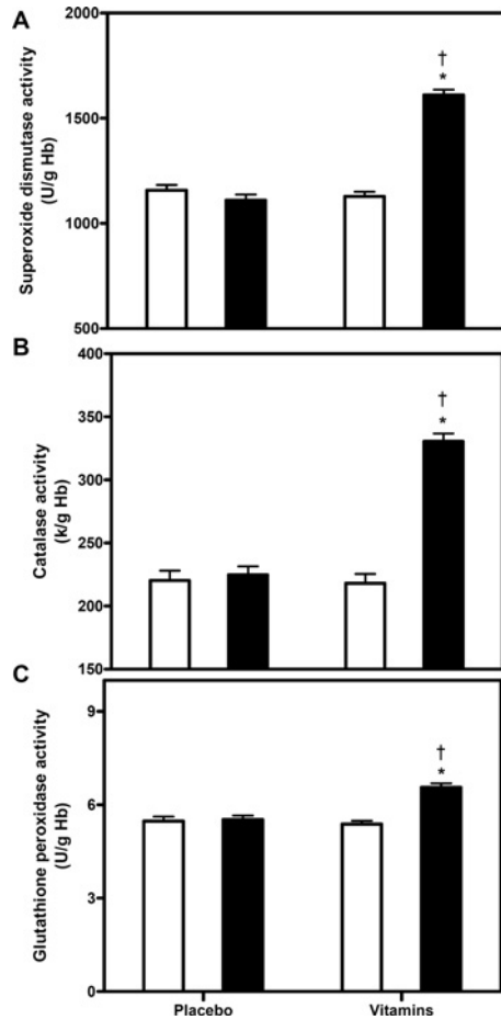
Figure 3 Activity of erythrocyte SOD (A), CAT (B) and GSH-Px (C) in patients with EH before (open bars) and after (closed bars) treatment with either vitamins C + E or placebo
