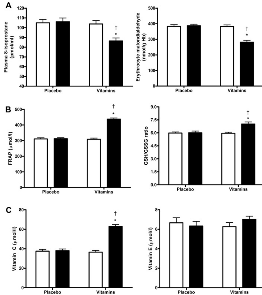
Figure 2 Lipid peroxidation (A) and antioxidant-capacity-related parameters (B and C) in patients with EH before (open bars) and after (closed bars) treatment with either vitamins C + E or placebo
