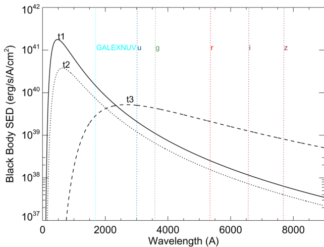
Figure 2. SEDs at three characteristic times for a standard NS10 model of a RSG progenitor with 500 R_{\odot} , 15 M_{\odot} and 1 foe. The mean wavelengths of filters NUV_{GALEX} and Sloan griz are shown.
