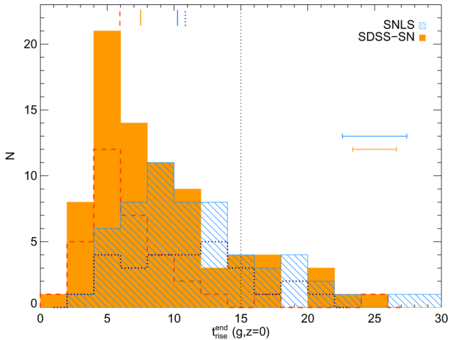
Figure 8. Histogram of t_{\text{rise}}^{\text{end}} rise-times at rest-frame g band ( \lambda_{\text{eff}} = 4722 \text{ \AA} ) for the silver samples of the SDSS-SN (solid orange) and SNLS (diagonal blue). The golden samples are shown in dashed and dotted lines, respectively. Median MC values are indicated with ticks at the top: 7.5^{+7.1}_{-3.6} and 6.0^{+3.8}_{-2.8} d for the silver and golden samples of the SDSS, and 10.3^{+7.8}_{-4.4} and 10.8^{+5.8}_{-5.1} d for the silver and golden samples of the SNLS, where the quoted uncertainties contain 84 per cent of the distribution. The vertical dotted line indicates the limit of long rise-time SNe (see Section 5.3). The horizontal error bar represent the typical median error on the rise of 2.5 d (SNLS) and 1.6 d (SDSS-SN).
