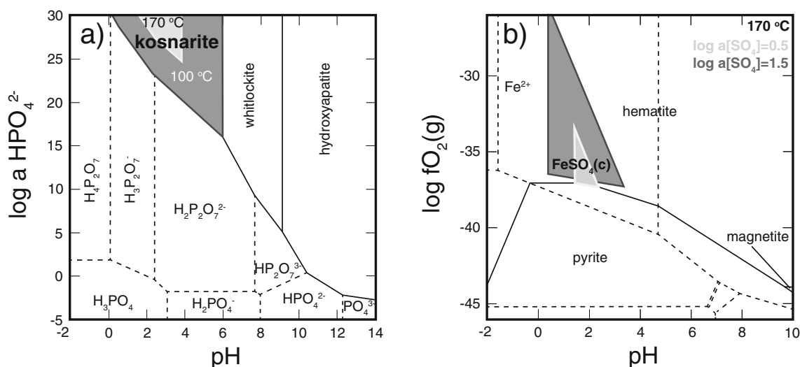
Fig. 3 Activity-pH diagrams showing stability conditions for a kosnarite and crystalline b FeSO 4 . a The \log a[\text{HPO}_4^{2-}] vs. pH diagram shows an expansion of the stability field of kosnarite when temperature decreases from 170 °C (bright gray) to 100 °C (dark gray). This change occurs at the expense of whitlockite and \text{H}_3\text{P}_2\text{O}_7 and \text{H}_2\text{P}_2\text{O}_7^{2-} aqueous species. Dashed lines show the stability fields of aqueous phosphate species. b Log f\text{O}_2 vs. pH diagram showing the stability field for FeSO 4 (approximating stability field of szomolnokite) and other Fe-bearing
