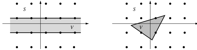
FIGURE 1. Two S -free sets for q = 2 .
