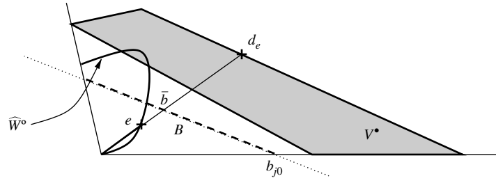
FIGURE 10. The extreme ray \mathbb{R}_+ b_{j_0} contains some point in V^* \setminus W^* .
