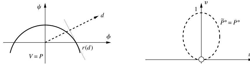
FIGURE 5. Trouble appears if the neighborhood has no asymptote.
