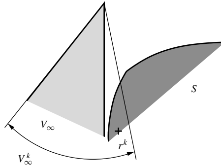
FIGURE 8. Constructing in S an unbounded sequence “tending to” V .
