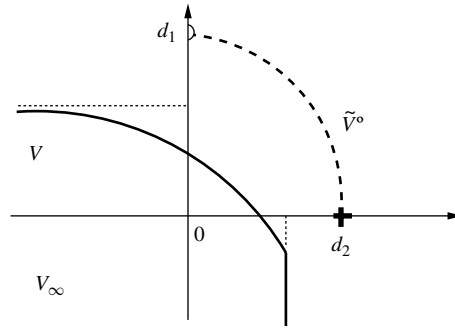
FIGURE 3. Activity in V^\circ .
