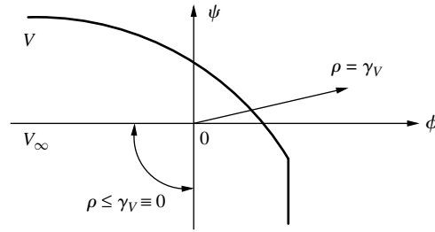
FIGURE 2. All representations coincide except in \text{int}(V_\infty) .
