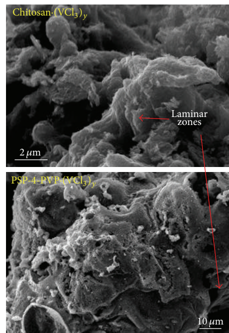
FIGURE 1: SEM image of pyrolytic products from PS-co-4-PVP·(VCl 3 ) y and chitosan·(VCl 3 ) y both in molar ratio 1:1. Red arrows indicate the underlying layered structure within the pyrolyzed material.
