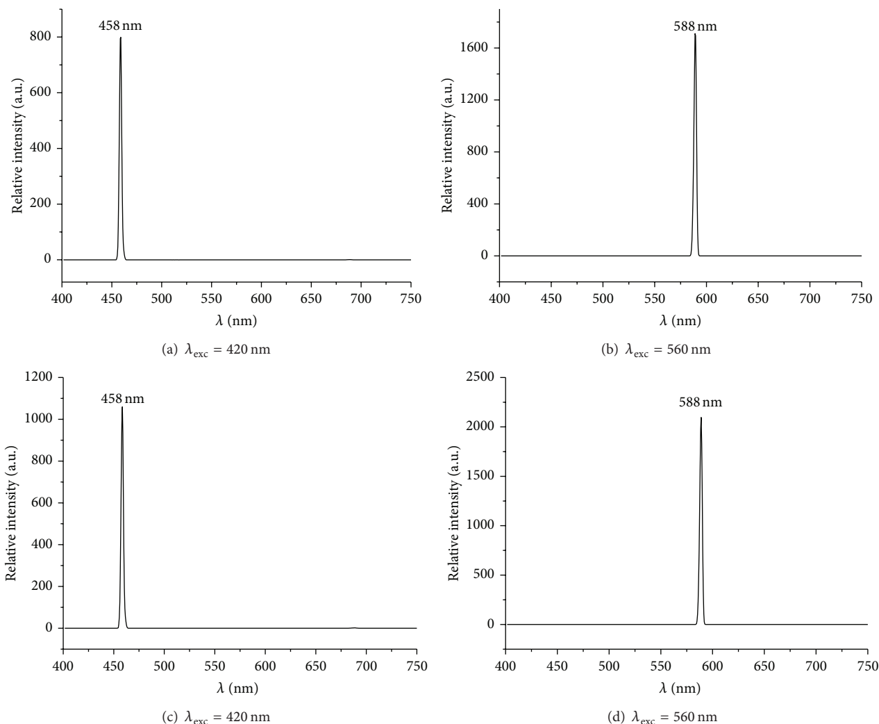
FIGURE 8: (a) Emission, (b) spectra of the pyrolytic products from \text{PS-co-4-PVP}\cdot(\text{VCl}_3)_y , and ((c), (d)) from pyrolytic products from \text{chitosan}\cdot(\text{VCl}_3)_y , at two different excitation energies.
