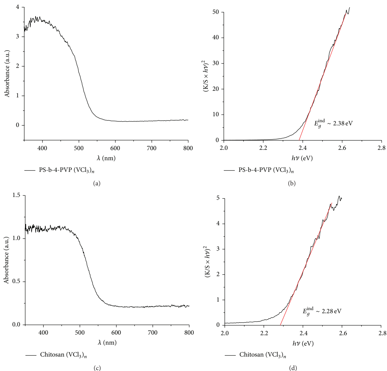
FIGURE 7: ((a), (c)) Absorption and ((b), (d)) Tauc et al. [56] plot of the pyrolytic products from PS-co-4-PVP·(VCl 3 ) y and chitosan·(VCl 3 ) y , respectively.
