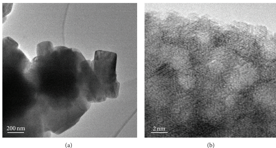
FIGURE 4: (a) TEM image of the pyrolytic precursor from 1:5 PS-co-4-PVP-(VCl 3 ) y and (b) HRTEM of a mesoporous laminar zone.
