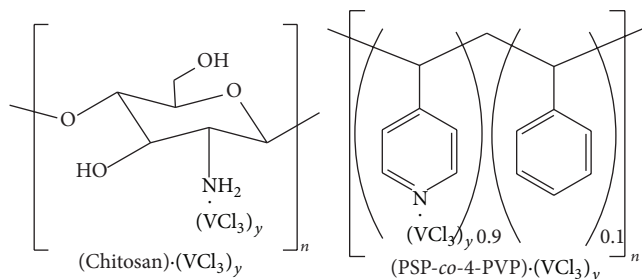
SCHEME 1: Representative formulas of chitosan and poly(styrene- co -4-vinylpyridine) and possible coordination sites of VCl 3 to the polymeric chain.
