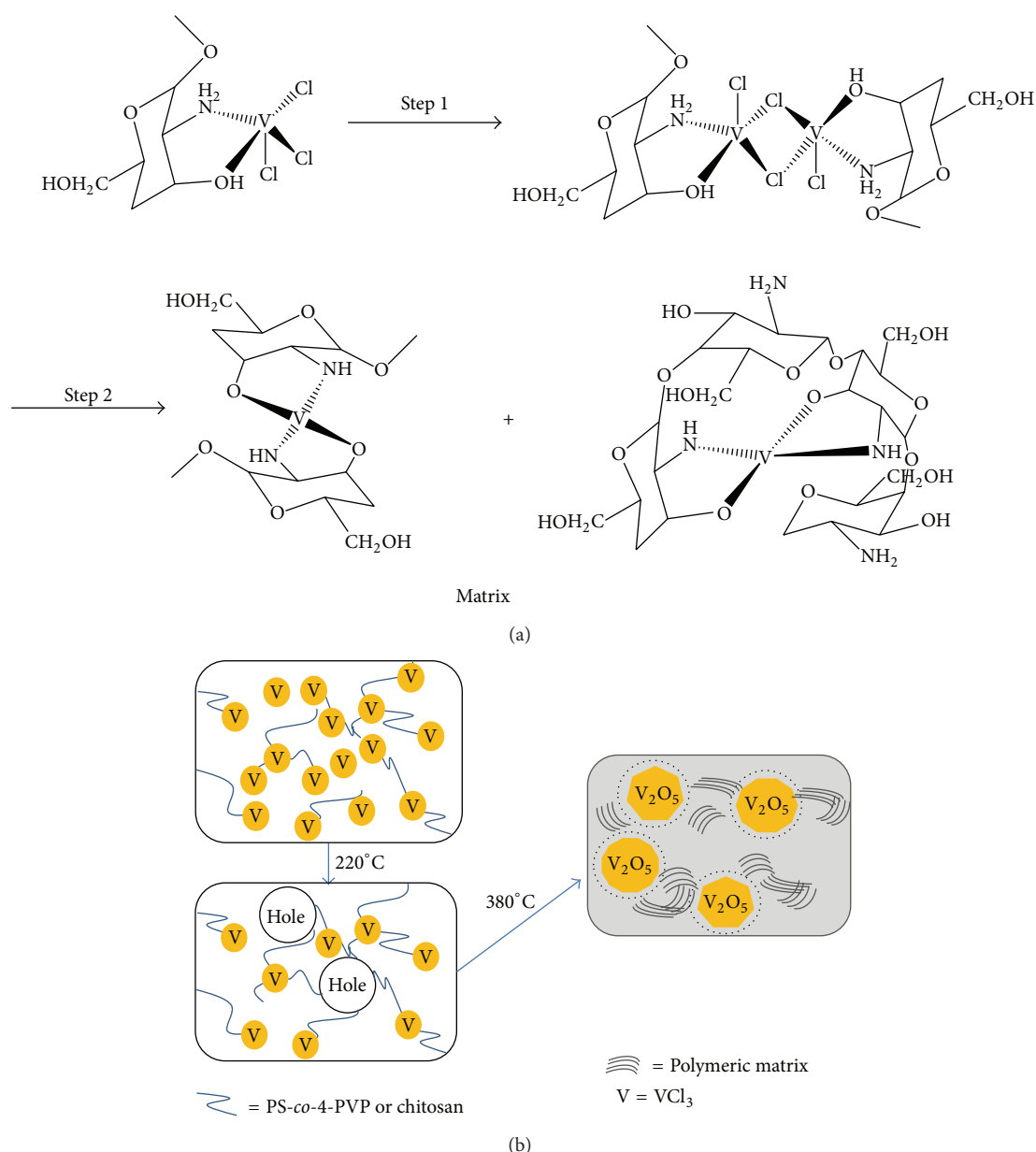
FIGURE 6: Possible coordination modes of the VCl_3 salt to the chitosan polymeric chain (a) and schematically proposed formation mechanism of the V_2O_5 materials and structures (b).
