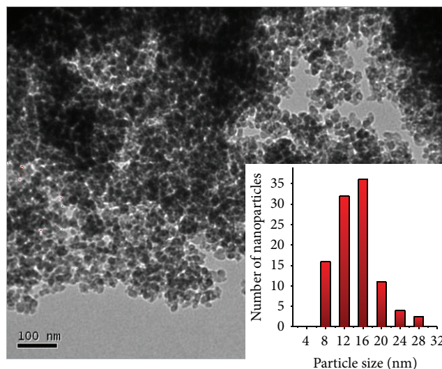
FIGURE 3: TEM image of pyrolytic product from chitosan·(VCl 3 ) y (1:5) and their histogram, inset.
