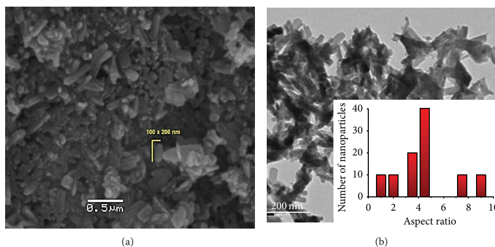
FIGURE 5: SEM (a) and TEM (b) image of the pyrolytic product from chitosan-(VCl 3 ) y (1:10) precursor.
