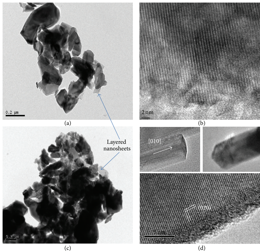
FIGURE 2: TEM and HRTEM images of the of pyrolytic products from ((a), (b)) 1:1 PS-co-4-PVP·(VCl 3 ) n and ((c), (d)) 1:1 chitosan·(VCl 3 ) n .
