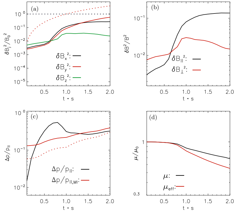
Figure 13. Magnetic field fluctuations, ion pressure anisotropy, and ion magnetic moment for a simulation with m_i/m_e = 10 , \beta_i = \beta_e = 20 , and \omega_{c,i}/s = 240 (run beta120magi240mass10). The ion results here are similar to the corresponding m_i = m_e results in Figures 7 and 9, indicating that the pair plasma results capture most of the key ion physics. Panel (a) shows the evolution of \delta B_j^2/B_0^2 and B_j^2/B_0^2 , in solid and dotted lines, respectively. The small contribution of \delta B_z^2 implies the dominance of mirror modes. Panel (b) shows the evolution of \delta B_{\perp}^2/B^2 (red) and \delta B_{\parallel}^2/B^2 (black) with \delta B_{\perp}^2 \gg \delta B_{\parallel}^2 , implying that the mirror modes have k_{\perp} \gg k_{\parallel} . Panel (c) shows the evolution of the ion pressure anisotropy \Delta p_i/p_{\parallel,i} (black-solid). The linear mirror threshold for mirror modes with \gamma/\omega_{c,i} = 0.05 in a \beta_i = \beta_e , m_i/m_e = 10 plasma is also shown (red line) along with the analogous threshold for m_i/m_e = 1836 for comparison (red dotted line). Panel (d) shows the evolution of \mu ( \equiv \langle v_{\perp,i}^2/B \rangle , black-solid) and \mu_{\text{eff}} ( \equiv \langle v_{\perp,i}^2 \rangle / \langle B \rangle , red-solid); see Equation (4) and associated text for details.
