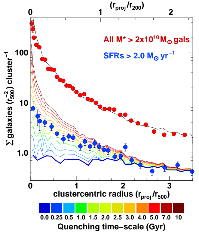
Figure 18. Blue symbols show the \Sigma(r) profile of \mathcal{M} > 2 \times 10^{10} M_{\odot} galaxies with obscured star formation at rates \text{SFR}_{\text{IR}} > 2.0 M_{\odot} \text{yr}^{-1} . Red symbols indicate the corresponding \Sigma(r) profile for all \mathcal{M} > 2 \times 10^{10} M_{\odot} galaxies. The thick blue curve shows the predicted surface density profile of infalling galaxies yet to pass within r_{200} , normalized to fit the observed surface density profile of star-forming galaxies at large radii. The remaining colored curves show the predicted surface density profiles for star-forming galaxies accreted into the clusters and subsequently have their star-formation rates decline exponentially with a range of quenching time-scales ( t_Q = 0.25 –10 Gyr).
