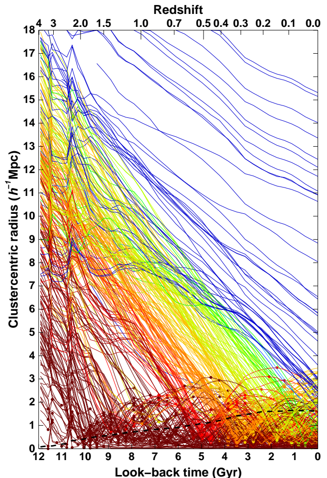
Figure 10. The infall of galaxies onto a massive cluster. Each galaxy with \mathcal{M} > 2 \times 10^{10} M_{\odot} at z=0 is shown by a colored curve tracing its comoving cluster-centric distance as a function of look-back time. The curves are color coded according to the epoch at which the galaxy is accreted into the cluster, as in Figure 9. The first pericenter and apocenter of each galaxy's orbit about the cluster are marked with dots. The black dashed curve indicates the evolution of the cluster radius r_{200} with time. Only galaxies which would be spectroscopically identified as cluster members by the observer are shown.
