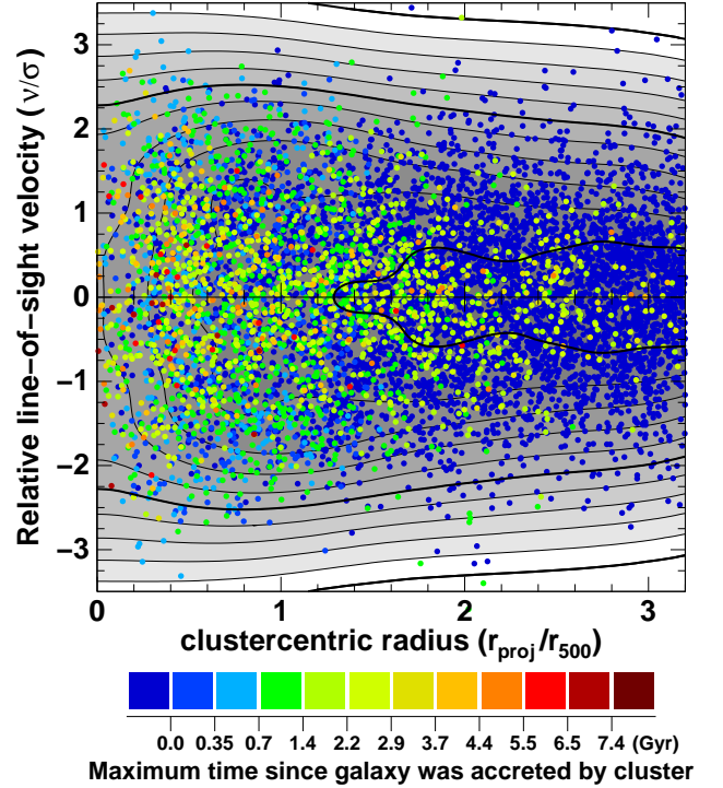
Figure 22. Stacked phase-space diagram, \Delta v_z/\sigma_v versus r_{proj}/r_{500} , for model star-forming galaxies around the 75 most massive clusters in the Millennium simulation at z=0.21 for the best-fit quenching model, in which star formation declines exponentially on a time-scale t_Q=1.73 Gyr in galaxies from the moment they pass within r_{200} of the cluster for the first time. Each point marks a M > 2 \times 10^{10} M_\odot star-forming galaxy with \text{SFR} > 2.0M_\odot \text{yr}^{-1} , colored according to time elapsed since it was accreted into the cluster (mid-blue if it is yet to be accreted). The grayscale contours indicate the resulting probability distribution function of the model star-forming galaxies in phase-space, P(r_{proj}/r_{500}, \Delta v_z/\sigma_v) . Each contour indicates a factor 0.2 dex change in phase-space density of model star-forming galaxies. The thick contours indicate a factor 10 change in phase-space density.
