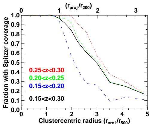
Figure 1. Radial coverage of the Spitzer /MIPS 24\mu\text{m} data. Each curve shows the fraction of cluster members covered by our 24\mu\text{m} images ( 25' \times 25' field-of-view) as a function of cluster-centric radius in units of r_{500} , for clusters in the following redshift ranges: 0.15 < z < 0.20 (long-dashed blue curves); 0.20 < z < 0.25 (dot-dashed green curves); 0.25 < z < 0.30 (short-dashed red curves); 0.15 < z < 0.30 (solid black curves).
