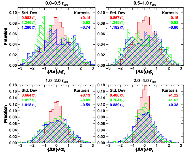
Figure 20. Stacked relative LOS velocity distributions of “spectroscopic” cluster galaxies for the 75 most massive clusters in the Millennium simulation at z=0.21 split into three dynamic sub-populations: (i) infalling “spectroscopic” cluster members yet to reach pericenter ( blue striped histogram ); (ii) back-splash galaxies which have passed through pericenter, are on their way back out of the cluster v_{radial} > 0 , and are yet to reach apocenter ( green striped histogram ); and (iii) the virialized cluster population which has passed through apocenter ( red solid histogram ). Each panel represents a different bin in cluster-centric radius as in Fig. 7. The standard deviations (in units of \sigma_v ) and kurtosis values of each distribution are indicated.
