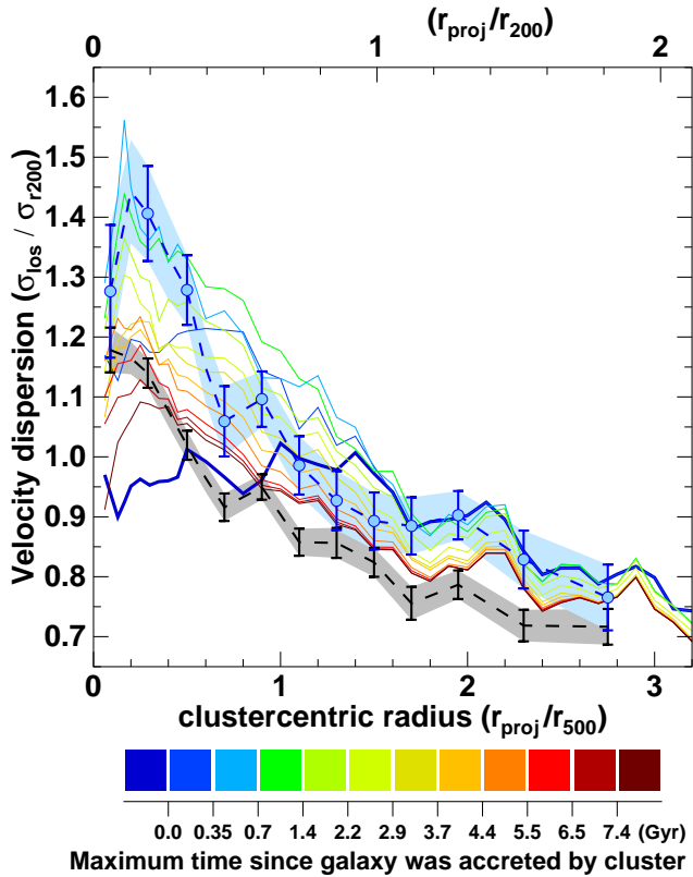
Figure 19. Predicted velocity dispersion profiles as a function of accretion epoch for model galaxies in our stacked sample of 75 clusters from the Millennium simulation at z=0.21 . The thick blue curve shows the predicted LOS velocity dispersion profile of “spectroscopic” cluster members yet to pass within r_{200} and be accreted into the cluster DM halo. The remaining solid curves show the impact on the velocity dispersion of progressively including those galaxies accreted into the clusters within the last \Delta t Gyr as indicated by the color scale. The black solid curve shows the velocity dispersion profile obtained by including all cluster members. Blue symbols with error bars show the observed velocity dispersion profile of the 24\mu\text{m} -detected cluster members from our stacked sample of 30 clusters. The black dashed curve shows the corresponding profile considering all \mathcal{M} > 2 \times 10^{10} M_{\odot} cluster members.
