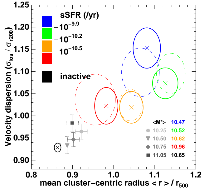
Figure 8. Variation in the spatial distribution and kinematics of cluster galaxies as a function of their specific-SFR and stellar mass. Colored crosses indicate the mean cluster-centric radii ( \langle r_{proj}/r_{500} \rangle ) and LOS velocity dispersions ( \sigma_{los}(r_{proj} < 2.0r_{500})/\sigma_\nu ) of star-forming cluster galaxies split into four bins of specific-SFR. Error ellipses show the 1\sigma uncertainties in both values. The black cross indicates the corresponding values for inactive cluster galaxies not detected with Spitzer . Only cluster galaxies within 2r_{500} are included within each sub-sample. The mean stellar mass, \langle \log(M/M_\odot) \rangle , of each sub-sample is indicated in the lower-right corner. Thin dashed ellipses indicate the results after applying additional stellar mass cuts to each specific-SFR bin to equalize their mean stellar masses to that of the inactive population. Grayscale symbols and error-bars indicate the mean cluster-centric radii and LOS velocity dispersions of cluster galaxies (including both star-forming and inactive sub-populations) split into four bins of stellar mass: \log(M/M_\odot) < 10.4 (light gray circle); 10.4 < \log M < 10.6 (gray triangle); 10.6 < \log M < 10.85 (mid-gray diamond); \log M > 10.85 (dark-gray square). ulation into bins of stellar mass ( grayscale symbols ), much less variation in the mean radii and LOS velocity dispersions is seen between stellar mass bins in comparison to those split by specific-SFR, and no overall trend with stellar mass is visible. Moreover, the kinematic segregation by specific-SFR persists even if additional stellar mass cuts are applied to each specific-SFR bin to equalize their mean stellar masses ( thin dashed ellipses ).
