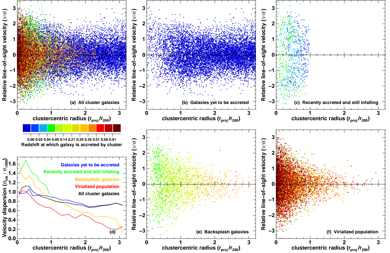
Figure 13. Stacked phase-space diagram ( \Delta v_{\text{los}}/\sigma_{\nu} vs. r_{\text{proj}}/r_{200} ) for the 75 most massive clusters in the Millennium simulation at z=0.0 (panel a). Each point indicates an \mathcal{M} > 2 \times 10^{10} M_{\odot} galaxy from the Bower et al. (2006) semi-analytic model catalog, colored according to when it was accreted onto the cluster. The four panels on the right split these cluster galaxies into dynamical sub-populations: (b) just those galaxies yet to pass within r_{200} and be accreted into the cluster; (c) infalling galaxies ( v_{\text{radial}} < 0 ) which have passed within r_{200} , but have yet to reach pericenter; (e) back-splash galaxies which have passed through pericenter and are on their way back out of the cluster ( v_{\text{radial}} > 0 ) and are yet to reach apocenter; (f) the virialized cluster population which have passed through apocenter. The lower left panel (d) displays the velocity dispersion profiles ( \sigma_{\text{los}}(r)/\sigma_{\nu} ) of each sub-population as well as that of the overall cluster population.
