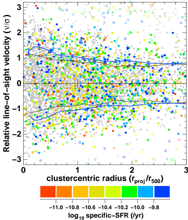
Figure 6. Stacked observed phase-space diagram, (\nu_{los} - \langle \nu \rangle) / \sigma_\nu versus r_{proj}/r_{500} , of galaxies combining all 30 clusters in our sample. Each gray solid dot represents a spectroscopic cluster member, while open points indicate non-cluster galaxies. Only those galaxies covered by our Spitzer data are plotted. Star-forming galaxies detected at 24\mu\text{m} are indicated by larger symbols, colored according to their specific-SFRs from red ( \text{sSFR} < 10^{-11} \text{ yr}^{-1} ) to blue ( \text{sSFR} > 10^{-10} \text{ yr}^{-1} ). The blue curve and error bars indicates the 1\text{-}\sigma velocity dispersion profile of the 24\mu\text{m} -detected cluster members. The uncertainty in each \sigma(r) value is estimated by bootstrap resampling the galaxies in that radial bin. The black curve shows the corresponding radial profile for the remaining inactive cluster members.
