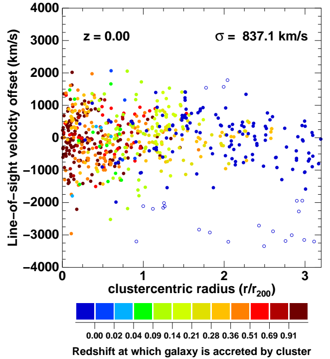
Figure 12. The caustic diagram ( \Delta v_{\text{los}} vs r_{\text{proj}}/r_{200} ) for M > 2 \times 10^{10} M_{\odot} galaxies orbiting around the same massive cluster, as viewed by distant observer along the z -axis. Galaxies are color coded according to their accretion epoch as in Figs. 9–11. Galaxies within 20 h^{-1} \text{ Mpc} of the cluster center at z=0.00 are indicated by solid symbols, while those at comoving cluster-centric radii r > 20 h^{-1} \text{ Mpc} are shown by open symbols. The velocity dispersion of galaxies within a projected cluster-centric radius r_{\text{proj}} < r_{200} is indicated.
