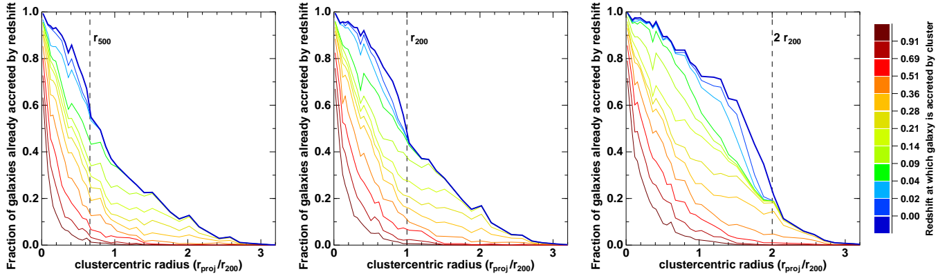
Figure 14. Radial population gradients in clusters. Each curve shows the fraction of “spectroscopic” cluster galaxies which have been accreted by a given redshift as a function of projected cluster-centric radius (normalized by r_{200} ) averaged over our stacked sample of 75 massive clusters observed at z=0.0 , color coded according to accretion redshift as indicated on the far right of the plot. The three panels indicate the trends produced when considering three definitions for describing when a galaxy is accreted into the cluster, taken to be the snapshot when the galaxy passes within r_{500} (left panel), r_{200} (middle panel) or 2r_{200} (right panel). The vertical dashed line in each panel indicates the corresponding radius at which the accretion epoch for the curves in that panel are defined.
