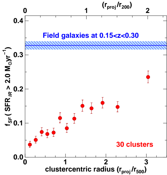
Figure 2. Radial population gradients for MIR-selected star forming galaxies from our stacked sample of 30 clusters. Red symbols show the fraction of massive ( M > 2.0 \times 10^{10} M_{\odot} ) cluster galaxies with obscured star-formation at rates SFR_{IR} > 2.0 M_{\odot} \text{ yr}^{-1} as a function of projected cluster-centric radius ( r_{proj}/r_{500} ). The error bars indicate the uncertainties derived from binomial statistics calculated using the formulae of Gehrels (1986). Each radial bin contains 400 cluster galaxies. The blue horizontal line indicates the corresponding fraction of field galaxies ( M > 2.0 \times 10^{10} M_{\odot} ; 0.15 < z < 0.30 ) with SFR_{IR} > 2.0 M_{\odot} \text{ yr}^{-1} and its 1\sigma confidence limits (shaded region).
