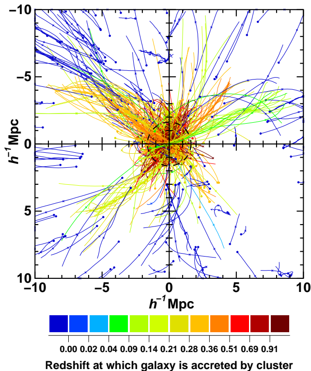
Figure 9. The orbits of galaxies about the 10th most massive cluster in the Millennium simulation, as viewed by a distant observer along the z -axis. The orbit of each galaxy with \mathcal{M} > 2 \times 10^{10} M_{\odot} at z=0 is shown by a colored curve, tracing its movement from z=0.76 (snapshot 44) to z=0.0 (snapshot 63). The final location of the galaxy is marked by a dot, while the cross indicates its location at z=0.41 (snapshot 50). Each curve is color coded according to the epoch at which the galaxy is accreted into the cluster, as indicated at the bottom of the plot. This accretion epoch is defined as the snapshot at which the galaxy passes within r_{200}(z) for the first time. Galaxies yet to pass within r_{200} have mid-blue colors, while those accreted earliest into the cluster ( z_{acc} > 0.51 ) have red colors. The dashed black circle indicates the present day r_{200} radius of the cluster. Only galaxies which would be spectroscopically identified as cluster members by the observer are shown.
