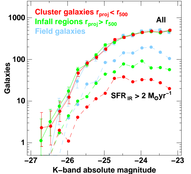
Figure 3. K -band luminosity functions (LFs) for cluster galaxies within r_{500} (red solid curve), galaxies from the infall regions ( r_{proj} > r_{500} ; green solid curve) and the coeval field population (light-blue solid curve). The latter two are normalized to contain the same total number of M_K < -23.1 galaxies as the cluster galaxy population, and the points slightly shifted horizontally, to permit easier comparison of the LFs. Error bars indicate Poissonian uncertainties based on Gehrels (1986). The corresponding K -band LFs for star-forming galaxies with SFR_{IR} > 2.0 M_{\odot} \text{ yr}^{-1} are indicated by dashed curves.
