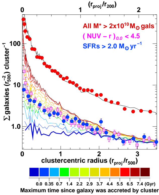
Figure 17. Blue symbols show the \Sigma(r) profile of \mathcal{M} > 2 \times 10^{10} M_{\odot} galaxies with obscured star formation at rates \text{SFR}_{\text{IR}} > 2.0 M_{\odot} \text{yr}^{-1} averaged over our 30 clusters. Magenta squares show the \Sigma(r) profile for unobscured star-forming galaxies with (\text{NUV}-r)_{0.0} < 4.5 , normalized to match the profile of obscured star-forming galaxies at r_{\text{proj}} \gtrsim 1.5 r_{500} . The thick blue curve shows the predicted surface density profile of infalling galaxies yet to pass within r_{200} , obtained from our “observations” of the 75 massive clusters in the Millennium simulation at z=0.21 , normalized to fit the observed radial profiles of star-forming galaxies at large radii. The remaining colored curves show the predicted radial profiles produced by including also those galaxies accreted into the clusters within the last \Delta t Gyr as indicated by the color scale. The black curve shows the predicted surface density profile for all “spectroscopic” member galaxies of the same 75 clusters, scaled to best match the observed ensemble \Sigma(r) profile of all \mathcal{M} > 2 \times 10^{10} M_{\odot} cluster galaxies (red points).
