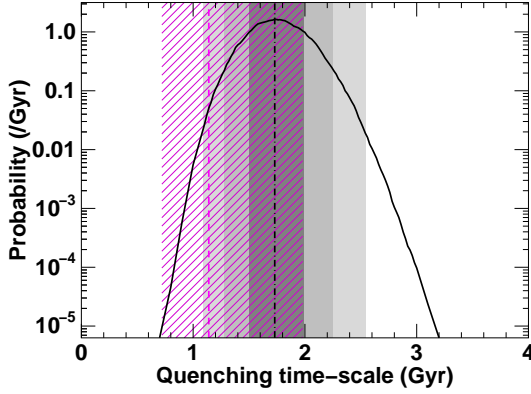
Figure 21. Likelihood function of the quenching time-scale, t_Q , based on fitting the distribution of star-forming galaxies in the caustic diagram, normalized so that \int \mathcal{L}(t_Q) = 1 with t_Q in units of Gyr. The best-fit value of t_Q is indicated by the vertical dot-dashed line, while the shaded regions indicate the 1, 2 and 3- \sigma confidence limits in t_Q . The magenta dashed line and hashed region indicates the best-fit t_Q value and 1- \sigma confidence limits by Haines et al. (2013) based on the systematically low specific-SFRs of star-forming cluster galaxies within r_{200} .
