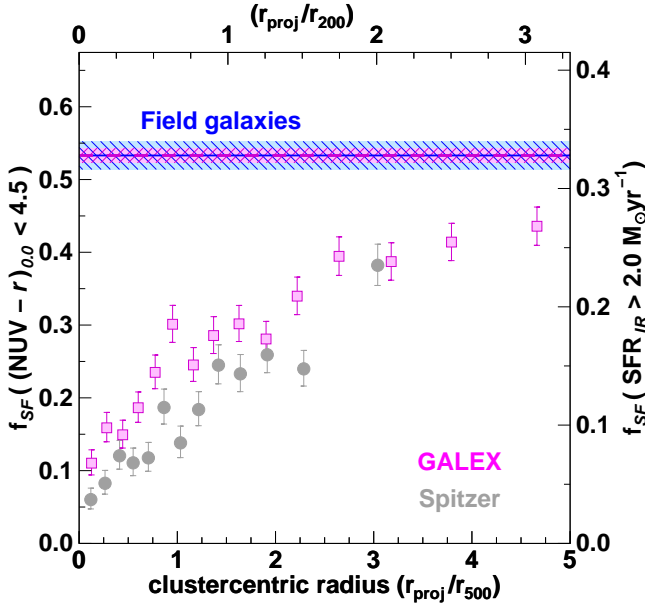
Figure 4. Comparison of radial population gradients for star-forming cluster galaxies selected in the ultraviolet and mid-infrared. Magenta squares show the fraction of massive ( M > 2.0 \times 10^{10} M_{\odot} ) cluster galaxies with blue rest-frame UV-optical colors, (NUV-r)_{0,0} < 4.5 , indicating ongoing unobscured star-formation. Each radial bin contains 300 cluster galaxies. The magenta dashed line indicates the corresponding fraction of field galaxies ( M > 2.0 \times 10^{10} M_{\odot} ; 0.15 < z < 0.30 ) with (NUV-r)_{0,0} < 4.5 and its 1\sigma confidence levels (magenta shaded region). Grey symbols show the corresponding fractions of cluster galaxies with SFR_{IR} > 2.0 M_{\odot} \text{ yr}^{-1} taken from Fig. 2, scaled via the right-hand axis, such that the fraction of field galaxies with SFR_{IR} > 2.0 M_{\odot} \text{ yr}^{-1} (blue dashed line) coincides with the corresponding fraction selected in the NUV.
