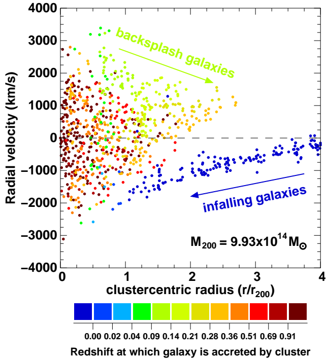
Figure 11. Radial phase-space diagram ( v_{\text{radial}} vs r/r_{200} ) for galaxies with M > 5 \times 10^9 M_{\odot} orbiting around the same massive cluster as in Figs 9 and 10. Galaxies are color coded according to their accretion epoch as indicated.
