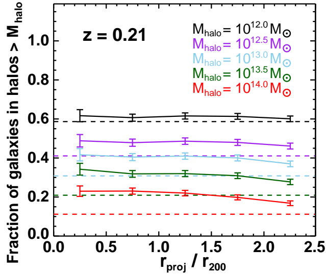
Figure 23. History bias for galaxies falling into massive clusters. The solid curves show the fraction of model galaxies surrounding massive clusters ( M_{cl} > 10^{14.2} M_{\odot} ) at z=0.21 which already reside in halos over a given mass as a function of projected cluster-centric radius. Only those galaxies yet to pass within r_{200} and be accreted into the cluster are included. The dashed curves show the corresponding cosmic fractions for field galaxies over the whole Millennium simulation.
