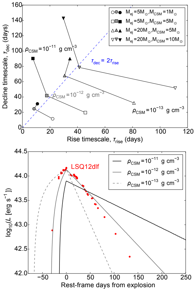
Figure 12. Rise vs decline timescales for synthetic light curves powered by ejecta-CSM interaction. The relation is strongly dependent on the density of the CSM. Models with \rho_{\text{CSM}} \sim 10^{-12} \text{ g cm}^{-3} (shown in Fig. 11) correspond best to our data. This can also be seen here in the lower panel, where we compare the SLSN LSQ12dlf to 3 models with M_{\text{ej}} = M_{\text{CSM}} = 5 M_{\odot} , and varying CSM density. The light curves peak when the forward shock from the ejecta-CSM collision breaks out of the CSM, and the subsequent decline is controlled mainly by the diffusion time in the CSM. Denser CSM results in faster shock propagation (shorter rise) and slower diffusion (longer decline), giving the inverse relationship between rise and decline times apparent in the top panel.
