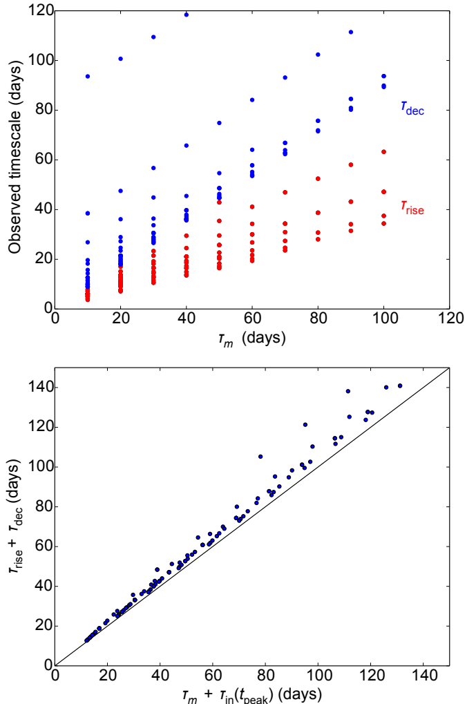
Figure 9. Same as Fig. 7, but for our magnetar model grid. The models shown have diffusion times of 10-100 d (steps of 10 d), B = \{1,3,5,7,9\} \times 10^{14} G, and P = \{1,3,5,7,9\} ms. Only models with peak luminosity greater than 3 \times 10^{43} ergs \text{s}^{-1} are plotted.
