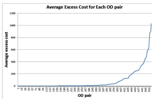
Figure 5. Optimality check.
