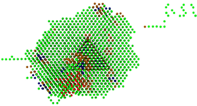
Fig. 3. Atoms in the final configuration, which are displaced more than a_0/\sqrt{2} with respect to their original position, viewed along [110]. Local crystalline structure is shown by the different colors (green: fcc; red: twin boundaries; blue: stacking faults, brown: unidentified atoms.). (For interpretation of the references to colour in this figure legend, the reader is referred to the web version of this article.)
