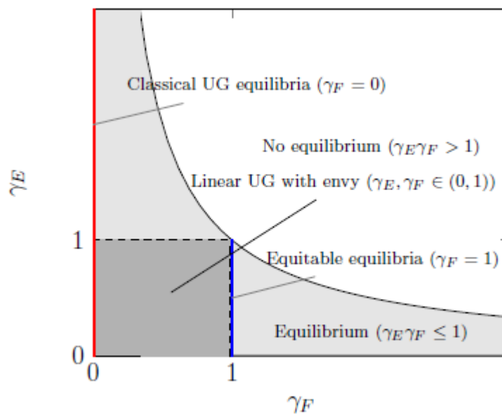
Figure 1. Equilibria of the Ultimatum Game (UG) with Externalities
