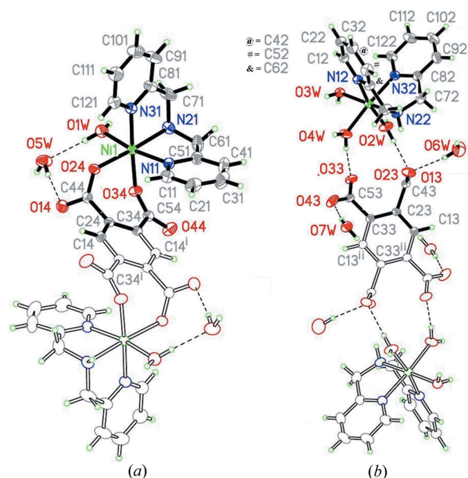
Figure 3 Molecular views of (II), showing (a) substructure C and (b) substructure S (both views expanded after application of the \bar{1} operation through the inversion centre at the btc^{4-} mid-point). Displacement ellipsoids are drawn at the 40% probability level and the symmetry-independent part of both substructures is shown with full bonds. [Symmetry codes: (i) -x + 1, -y + 2, -z + 1 ; (ii) -x + 1, -y + 2, -z .]
